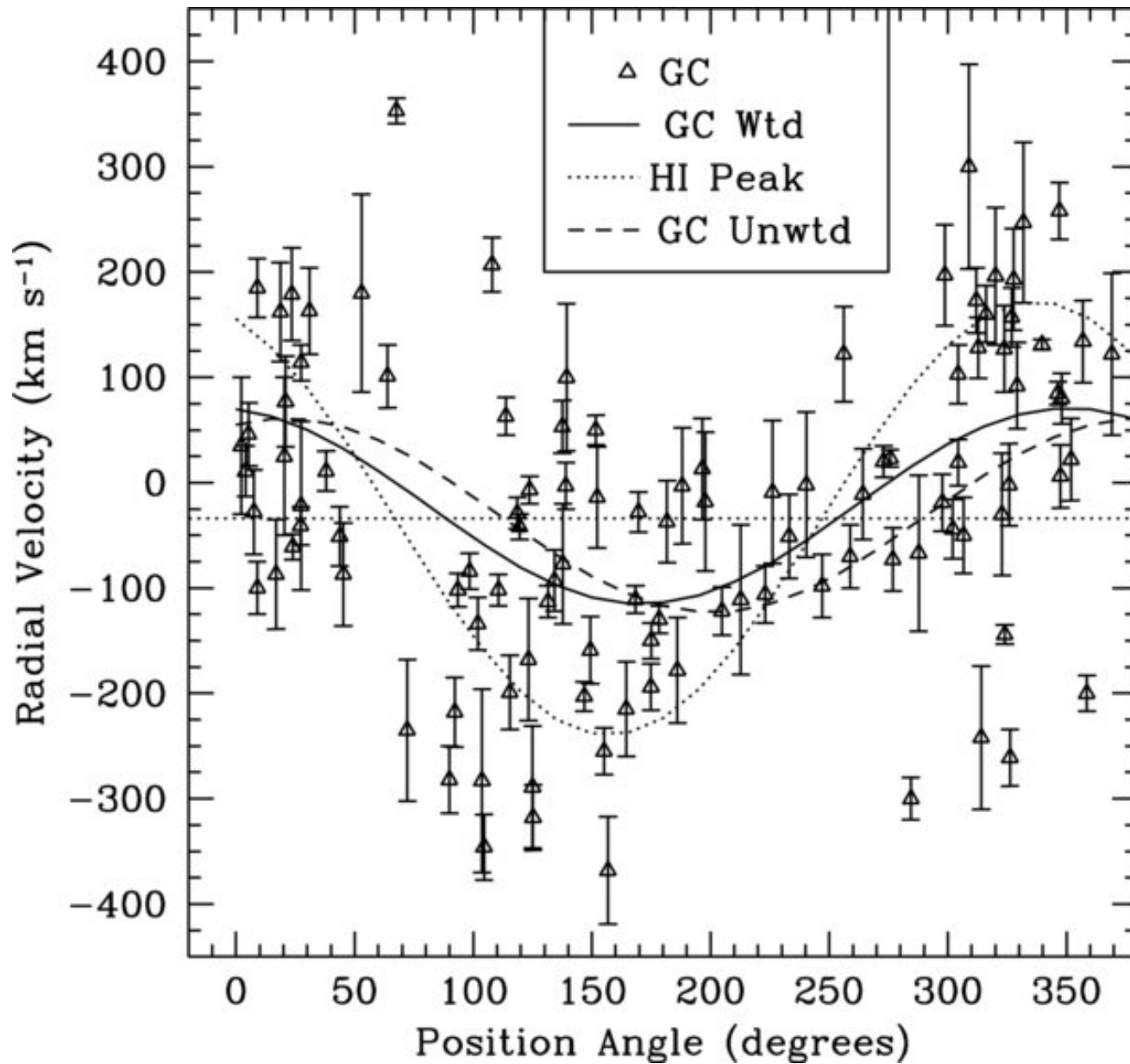
Figure 12. from Spectroscopy of M81 Globular Clusters NANTAIS & HUCHRA 2010 AJ 139 2620 doi:10.1088/0004-6256/139/6/2620 https://dx.doi.org/10.1088/0004-6256/139/6/2620 © 2010. The American Astronomical Society. All rights reserved.
