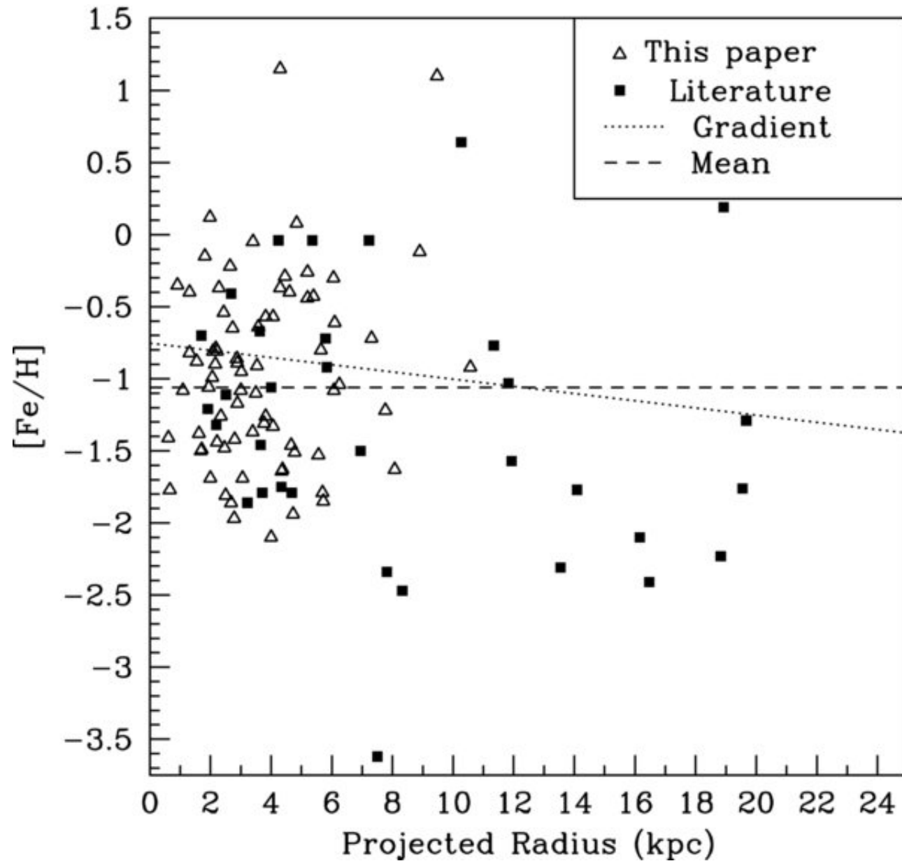
Figure 10. from Spectroscopy of M81 Globular Clusters NANTAIS & HUCHRA 2010 AJ 139 2620 doi:10.1088/0004-6256/139/6/2620 https://dx.doi.org/10.1088/0004-6256/139/6/2620 © 2010. The American Astronomical Society. All rights reserved.
