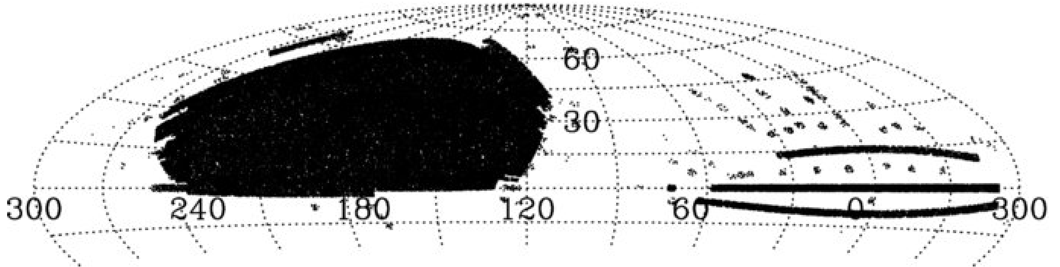
Figure 1. from The Sloan Digital Sky Survey Quasar Catalog. V. Seventh Data Release SCHNEIDER ET AL. 2010 AJ 139 2360 doi:10.1088/0004-6256/139/6/2360 https://dx.doi.org/10.1088/0004-6256/139/6/2360 © 2010. The American Astronomical Society. All rights reserved.
