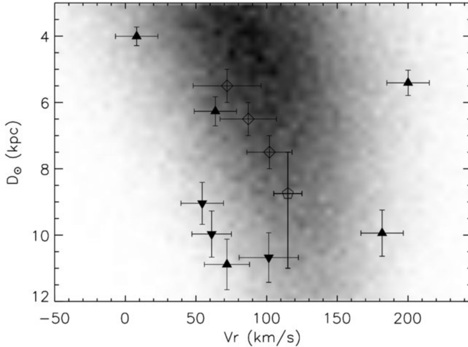
Figure 8. from No Excess of RR Lyrae Stars in the Canis Major Overdensity MATEU ET AL. 2009 AJ 137 4412 doi:10.1088/0004-6256/137/5/4412 https://dx.doi.org/10.1088/0004-6256/137/5/4412 © 2009. The American Astronomical Society. All rights reserved.
