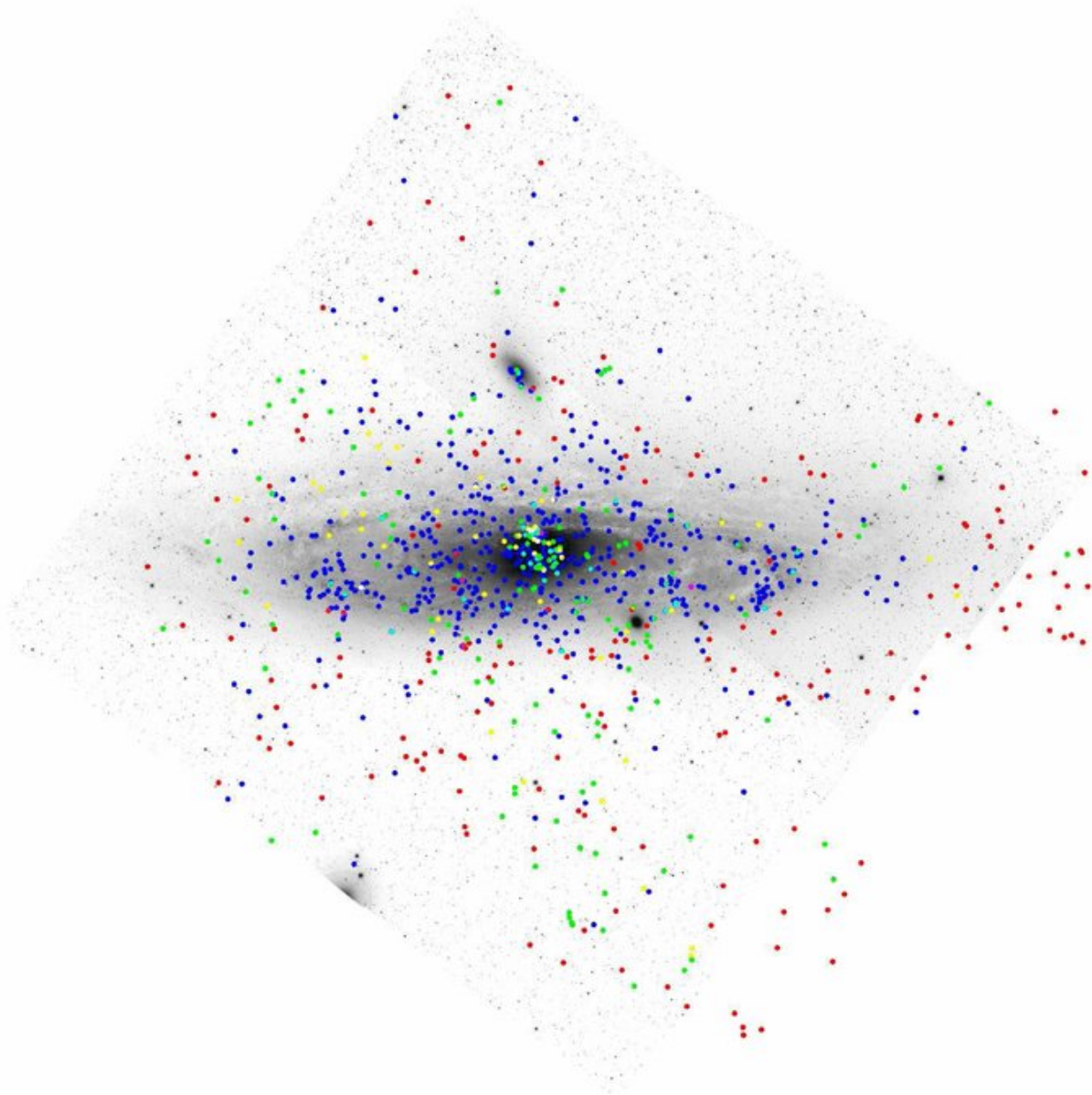
Figure 2. from Star Clusters in M31. I. A Catalog and a Study of the Young Clusters CALDWELL ET AL. 2009 AJ 137 94 doi:10.1088/0004-6256/137/1/94 https://dx.doi.org/10.1088/0004-6256/137/1/94 © 2009. The American Astronomical Society. All rights reserved.
