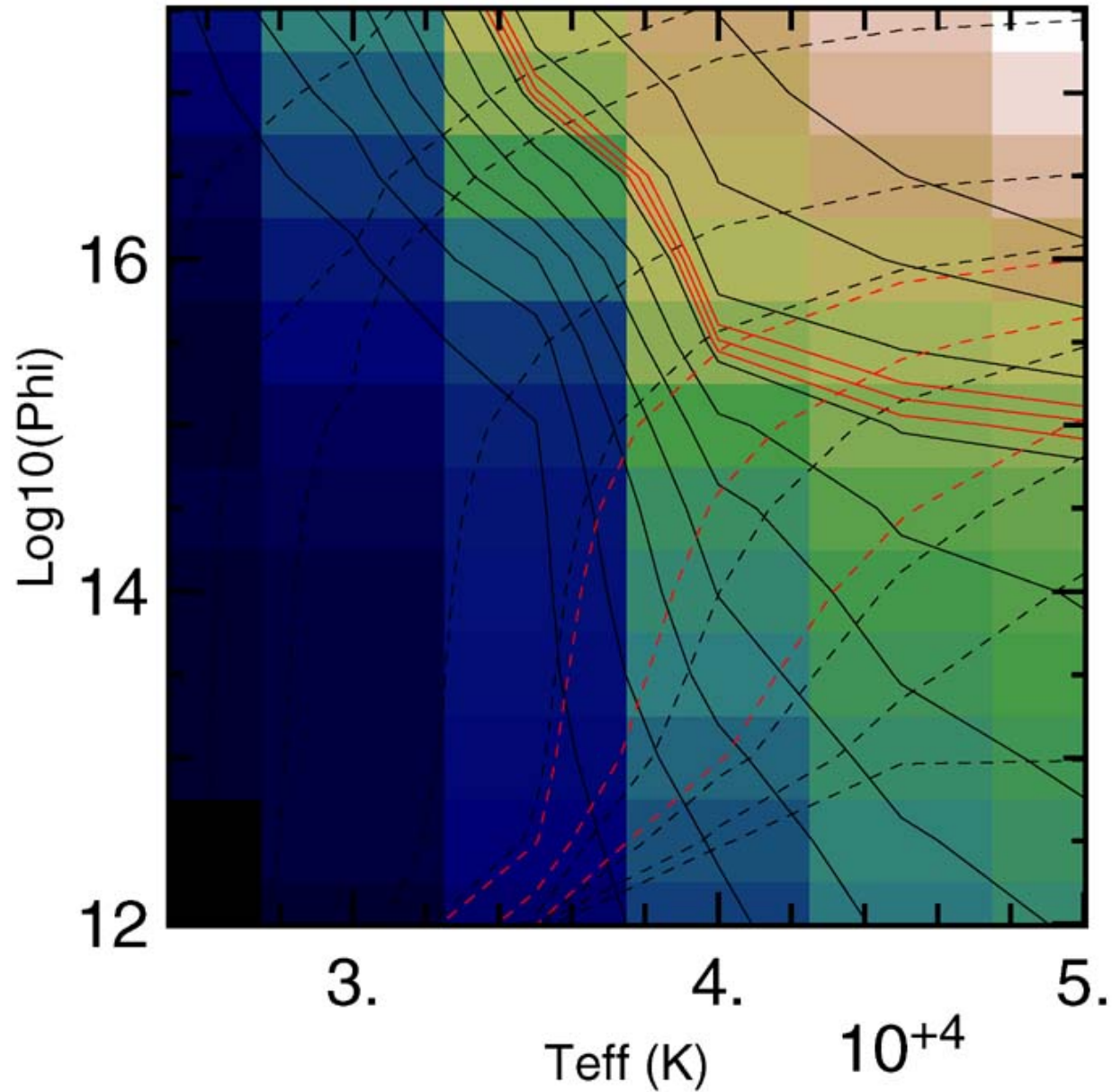
Figure 9. from The Ionizing Stars of the Galactic Ultra-Compact H II Region G45.45+0.06 BLUM & MCGREGOR 2008 AJ 135 1708 doi:10.1088/0004-6256/135/5/1708 https://dx.doi.org/10.1088/0004-6256/135/5/1708 © 2008. The American Astronomical Society. All rights reserved.
