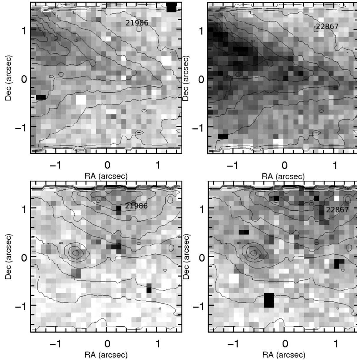
Figure 8. from The Ionizing Stars of the Galactic Ultra-Compact H II Region G45.45+0.06 BLUM & MCGREGOR 2008 AJ 135 1708 doi:10.1088/0004-6256/135/5/1708 https://dx.doi.org/10.1088/0004-6256/135/5/1708 © 2008. The American Astronomical Society. All rights reserved.
