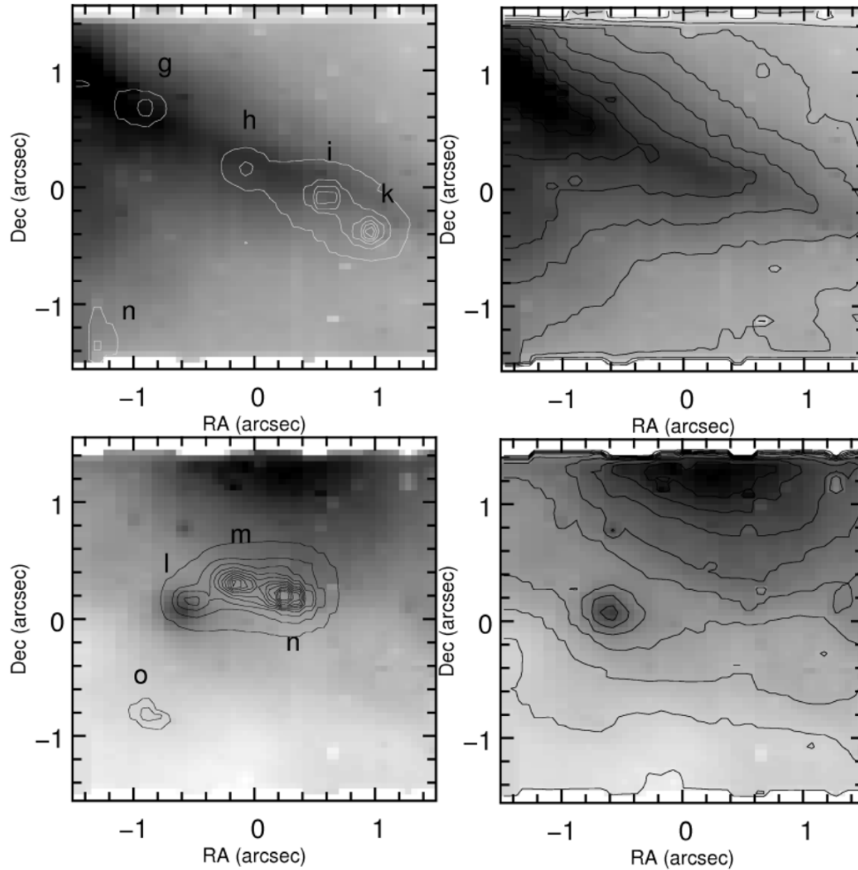
Figure 7. from The Ionizing Stars of the Galactic Ultra-Compact H II Region G45.45+0.06 BLUM & MCGREGOR 2008 AJ 135 1708 doi:10.1088/0004-6256/135/5/1708 https://dx.doi.org/10.1088/0004-6256/135/5/1708 © 2008. The American Astronomical Society. All rights reserved.
