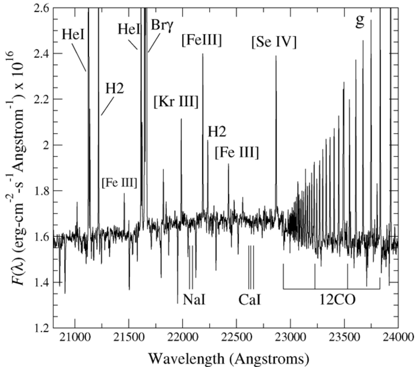
Figure 6. from The Ionizing Stars of the Galactic Ultra-Compact H II Region G45.45+0.06 BLUM & MCGREGOR 2008 AJ 135 1708 doi:10.1088/0004-6256/135/5/1708 https://dx.doi.org/10.1088/0004-6256/135/5/1708 © 2008. The American Astronomical Society. All rights reserved.
