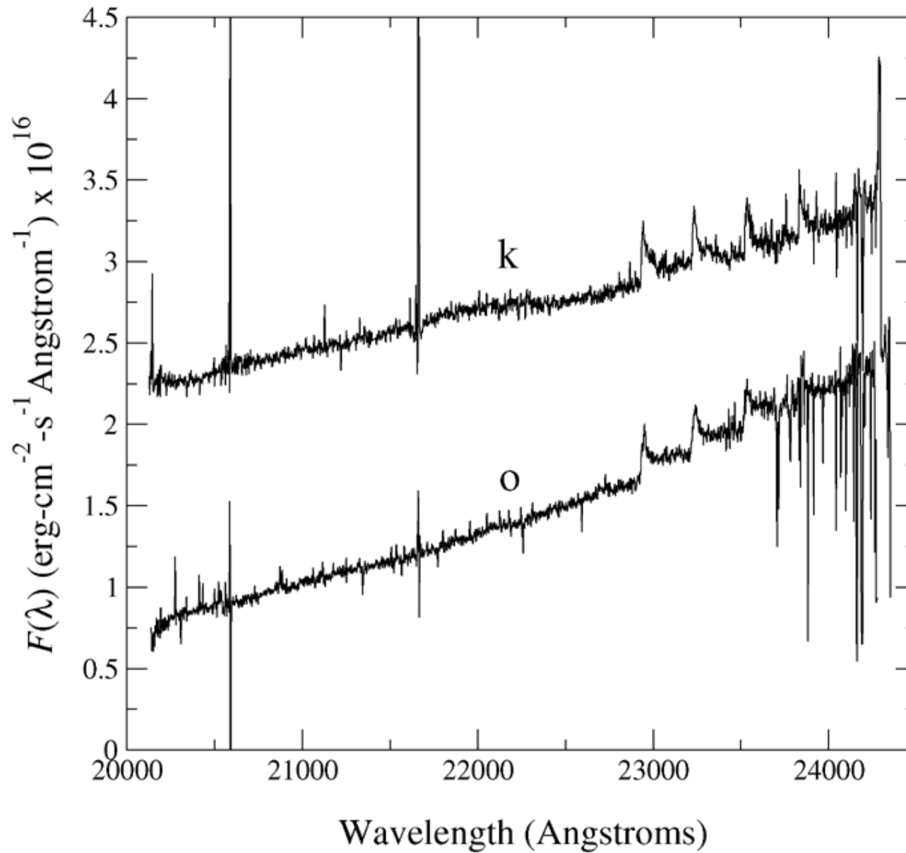
Figure 5. from The Ionizing Stars of the Galactic Ultra-Compact H II Region G45.45+0.06 BLUM & MCGREGOR 2008 AJ 135 1708 doi:10.1088/0004-6256/135/5/1708 https://dx.doi.org/10.1088/0004-6256/135/5/1708 © 2008. The American Astronomical Society. All rights reserved.
