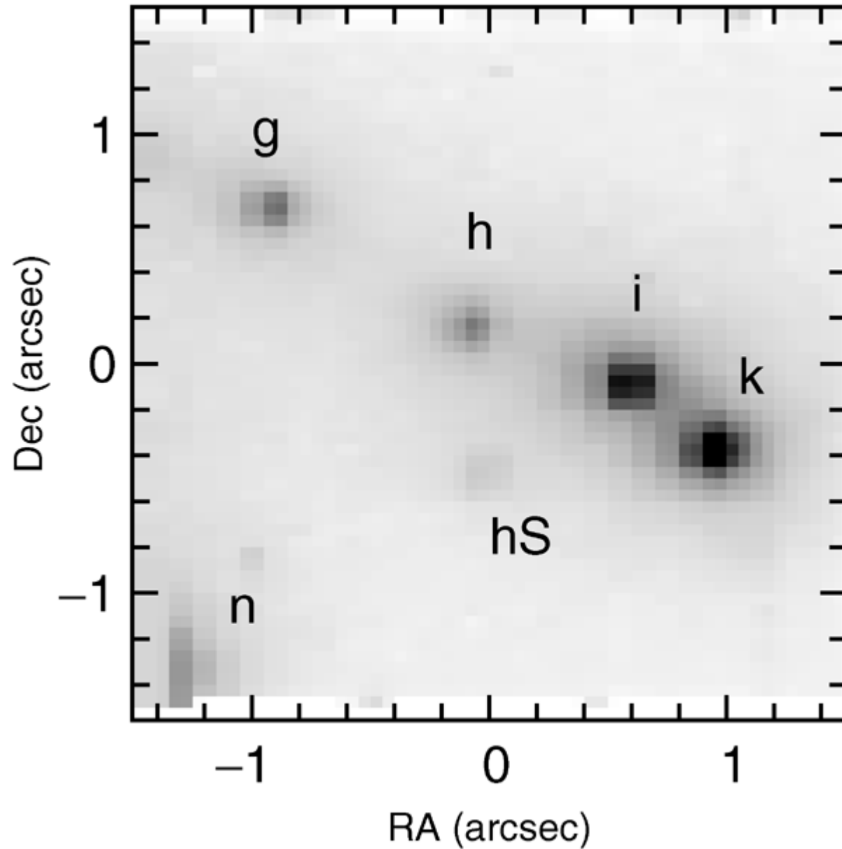
Figure 2. from The Ionizing Stars of the Galactic Ultra-Compact H II Region G45.45+0.06 BLUM & MCGREGOR 2008 AJ 135 1708 doi:10.1088/0004-6256/135/5/1708 https://dx.doi.org/10.1088/0004-6256/135/5/1708 © 2008. The American Astronomical Society. All rights reserved.
