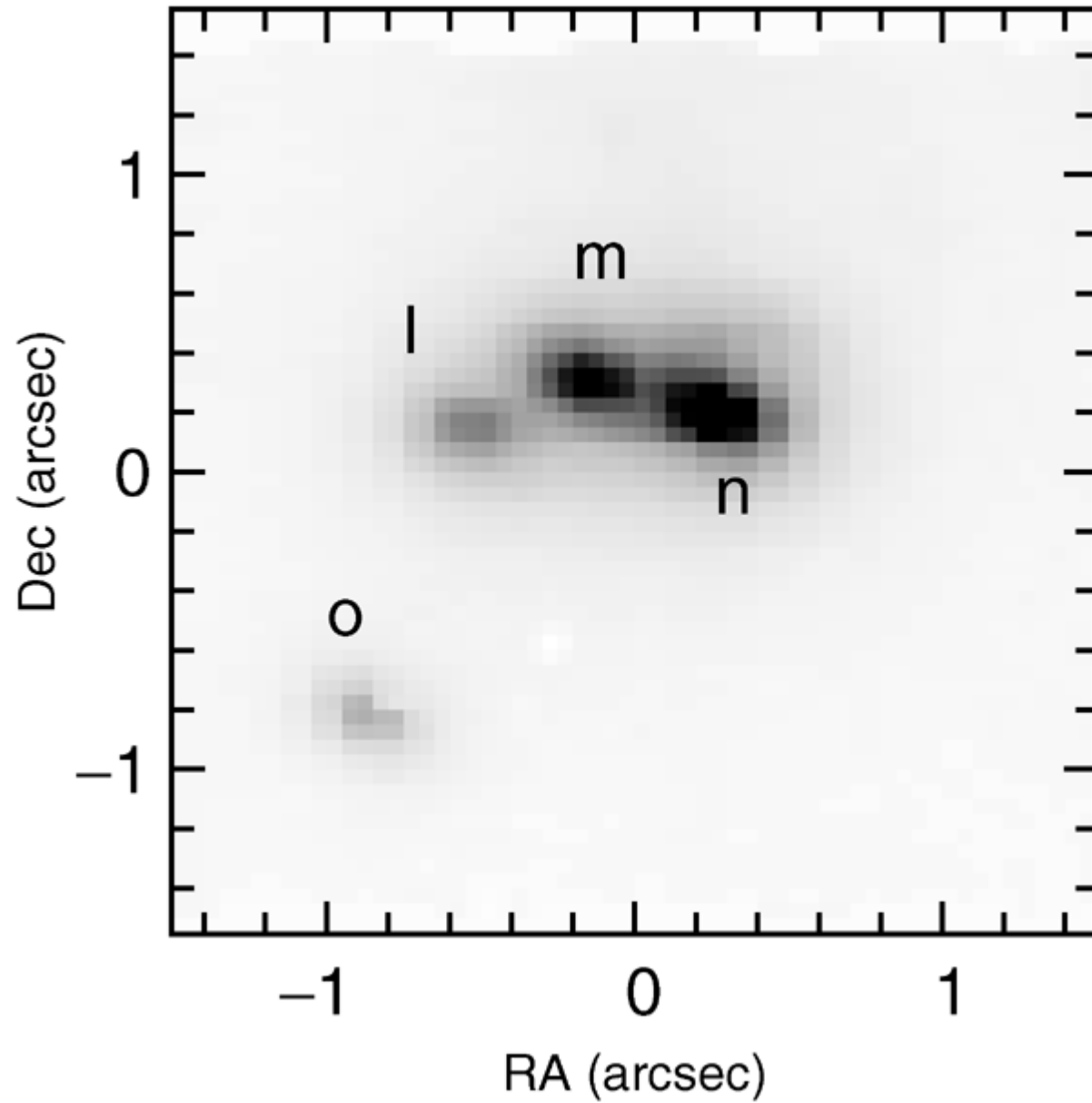
Figure 1. from The Ionizing Stars of the Galactic Ultra-Compact H II Region G45.45+0.06 BLUM & MCGREGOR 2008 AJ 135 1708 doi:10.1088/0004-6256/135/5/1708 https://dx.doi.org/10.1088/0004-6256/135/5/1708 © 2008. The American Astronomical Society. All rights reserved.
