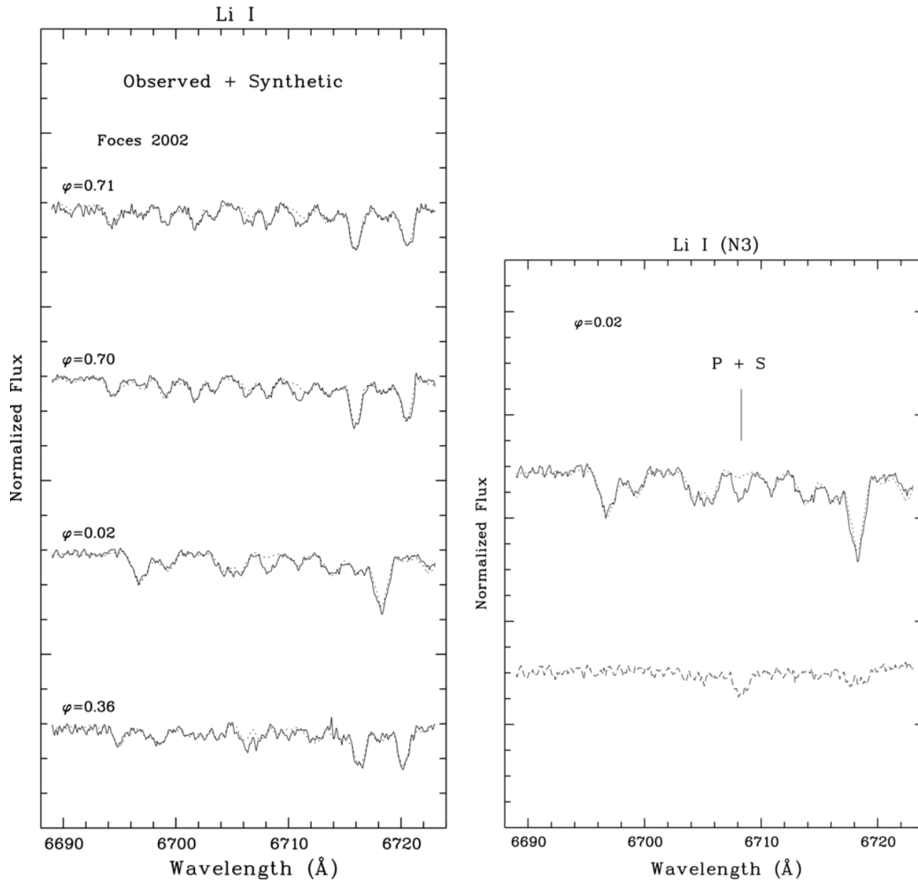
Figure 2. from Multiwavelength Optical Observations of Two Chromospherically Active Binary Systems: V789 Mon and GZ Leo GÁLVEZ ET AL. 2009 AJ 137 3965 doi:10.1088/0004-6256/137/4/3965 https://dx.doi.org/10.1088/0004-6256/137/4/3965 © 2009. The American Astronomical Society. All rights reserved.
