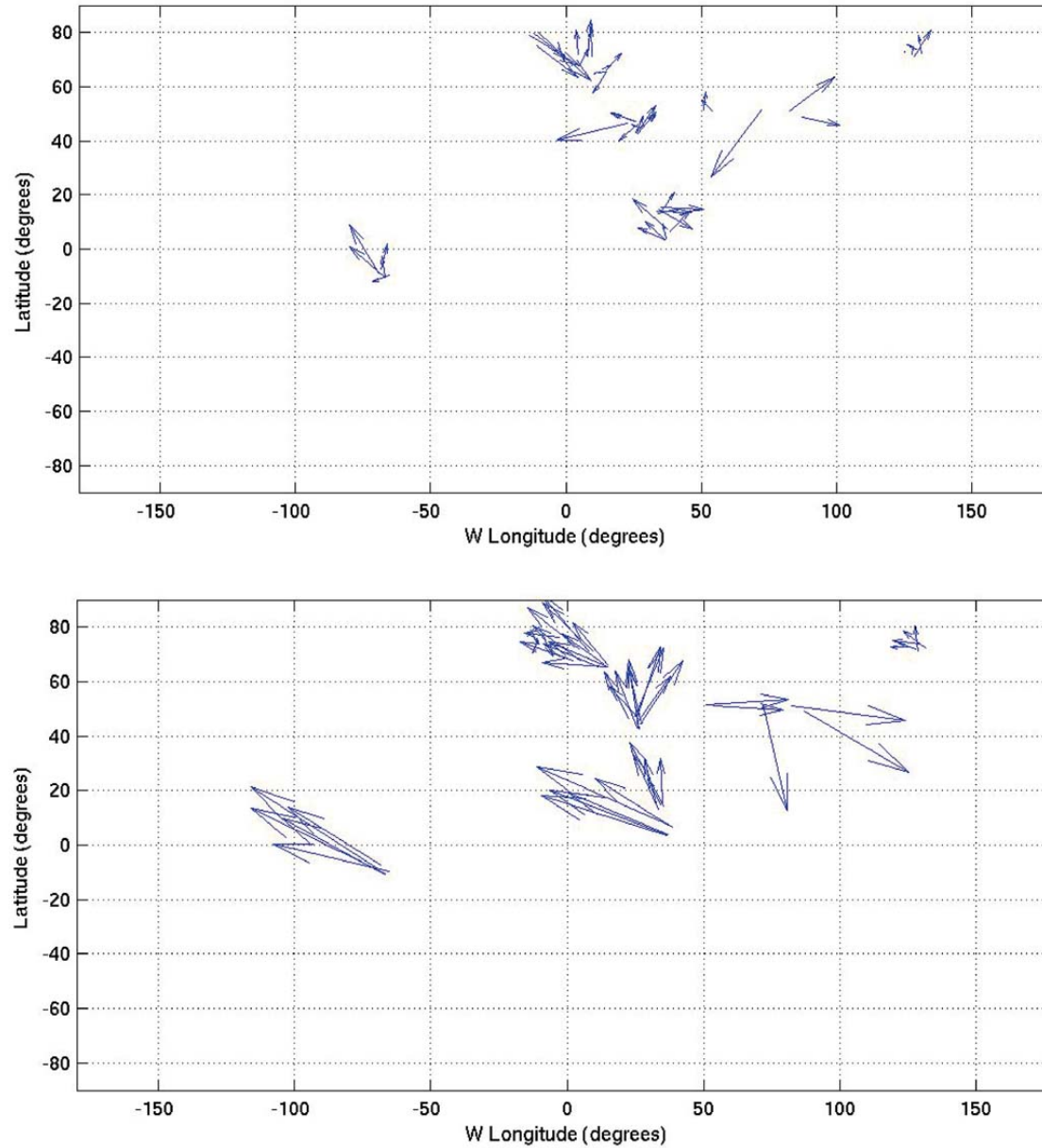
Figure 4. from Determining Titan's Spin State from Cassini RADAR Images STILES ET AL. 2008 AJ 135 1669 doi:10.1088/0004-6256/135/5/1669 https://dx.doi.org/10.1088/0004-6256/135/5/1669 © 2008. The American Astronomical Society. All rights reserved.
