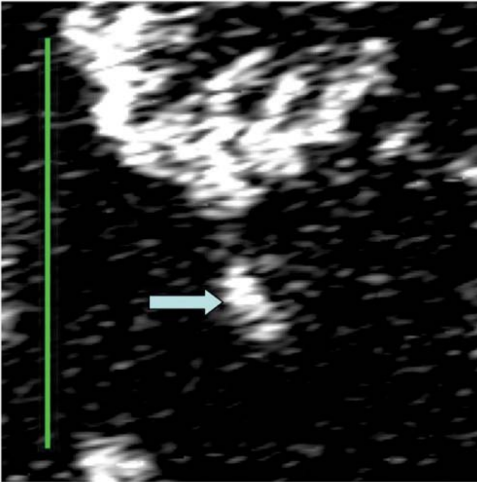
Figure 1. from Determining Titan's Spin State from Cassini RADAR Images STILES ET AL. 2008 AJ 135 1669 doi:10.1088/0004-6256/135/5/1669 https://dx.doi.org/10.1088/0004-6256/135/5/1669 © 2008. The American Astronomical Society. All rights reserved.
