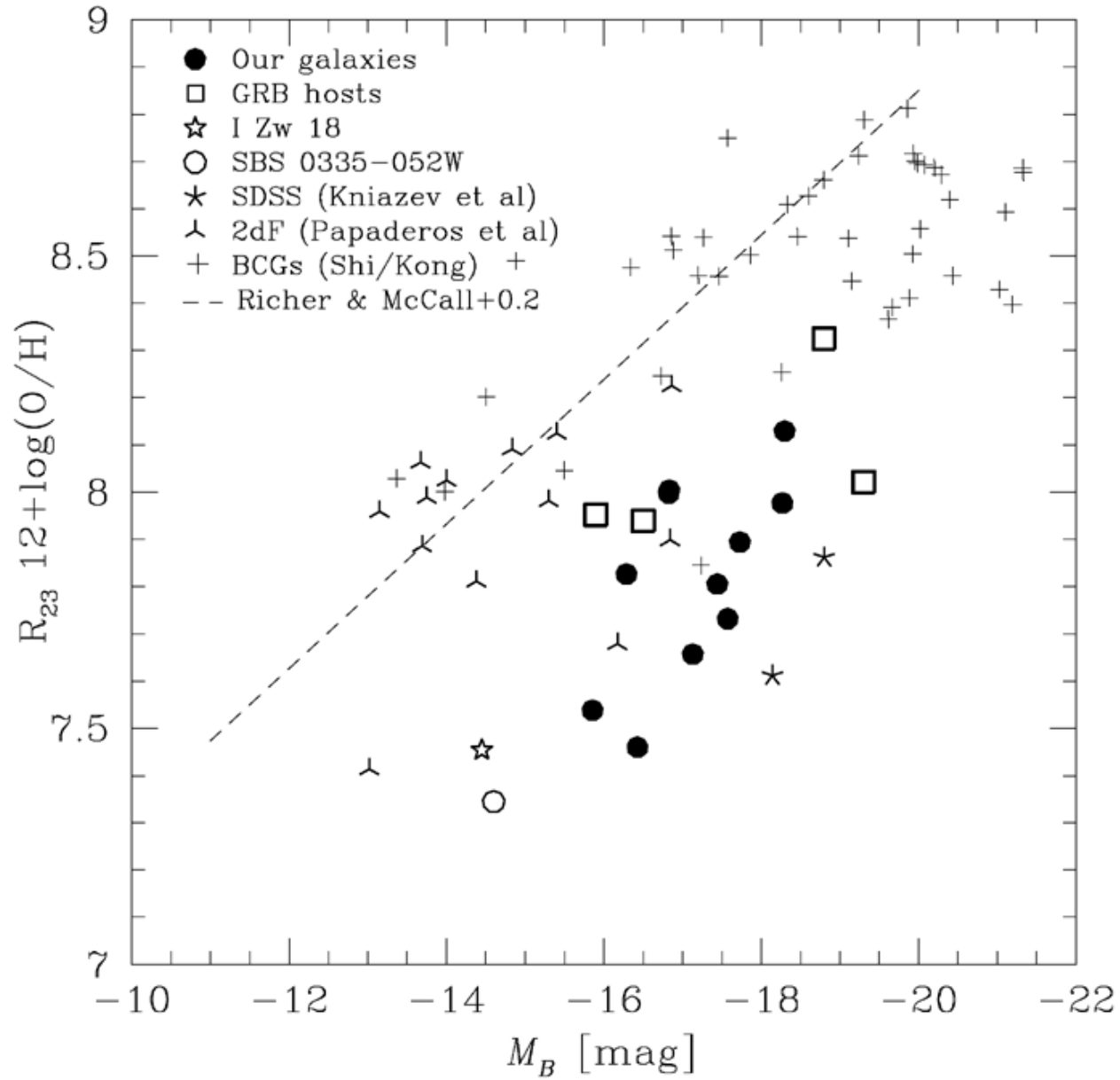
Figure 7. from MMT Extremely Metal-Poor Galaxy Survey. I. An Efficient Technique to Identify Metal-Poor Galaxies BROWN, KEWLEY, & GELLER 2008 AJ 135 92 doi:10.1088/0004-6256/135/1/92 https://dx.doi.org/10.1088/0004-6256/135/1/92 © 2008. The American Astronomical Society. All rights reserved.
