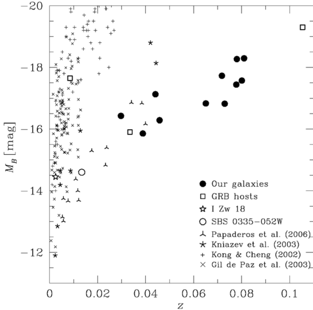
Figure 5. from MMT Extremely Metal-Poor Galaxy Survey. I. An Efficient Technique to Identify Metal-Poor Galaxies BROWN, KEWLEY, & GELLER 2008 AJ 135 92 doi:10.1088/0004-6256/135/1/92 https://dx.doi.org/10.1088/0004-6256/135/1/92 © 2008. The American Astronomical Society. All rights reserved.
