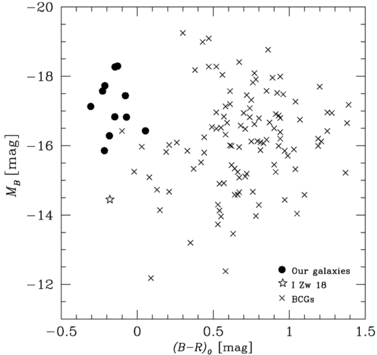
Figure 4. from MMT Extremely Metal-Poor Galaxy Survey. I. An Efficient Technique to Identify Metal-Poor Galaxies BROWN, KEWLEY, & GELLER 2008 AJ 135 92 doi:10.1088/0004-6256/135/1/92 https://dx.doi.org/10.1088/0004-6256/135/1/92 © 2008. The American Astronomical Society. All rights reserved.
