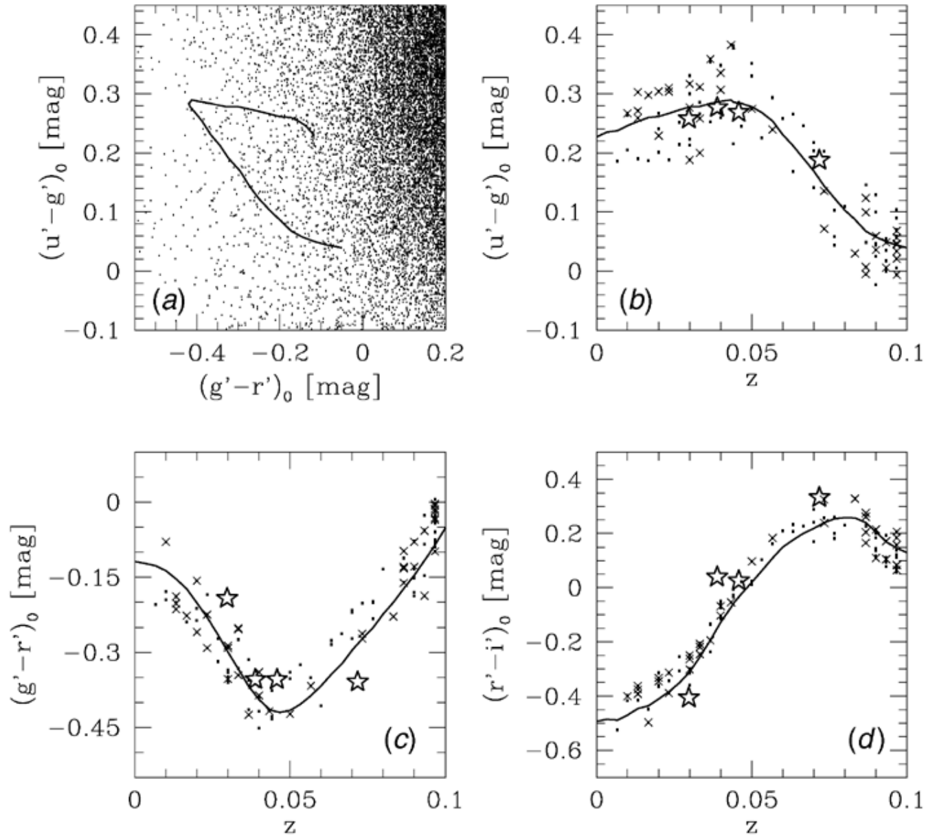
Figure 2. from MMT Extremely Metal-Poor Galaxy Survey. I. An Efficient Technique to Identify Metal-Poor Galaxies BROWN, KEWLEY, & GELLER 2008 AJ 135 92 doi:10.1088/0004-6256/135/1/92 https://dx.doi.org/10.1088/0004-6256/135/1/92 © 2008. The American Astronomical Society. All rights reserved.
