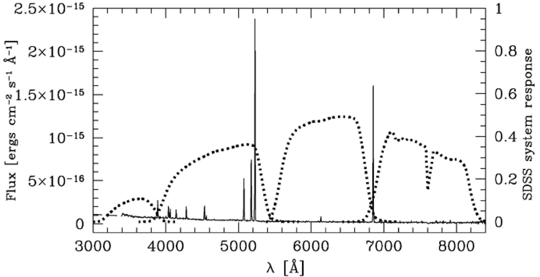
Figure 1. from MMT Extremely Metal-Poor Galaxy Survey. I. An Efficient Technique to Identify Metal-Poor Galaxies BROWN, KEWLEY, & GELLER 2008 AJ 135 92 doi:10.1088/0004-6256/135/1/92 https://dx.doi.org/10.1088/0004-6256/135/1/92 © 2008. The American Astronomical Society. All rights reserved.
