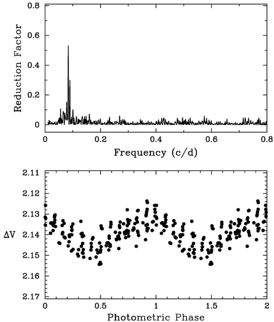
Figure 2. from The Rotation Period of the Planet-Hosting Star HD 189733 HENRY & WINN 2008 AJ 135 68 doi:10.1088/0004-6256/135/1/68 https://dx.doi.org/10.1088/0004-6256/135/1/68 © 2008. The American Astronomical Society. All rights reserved.
