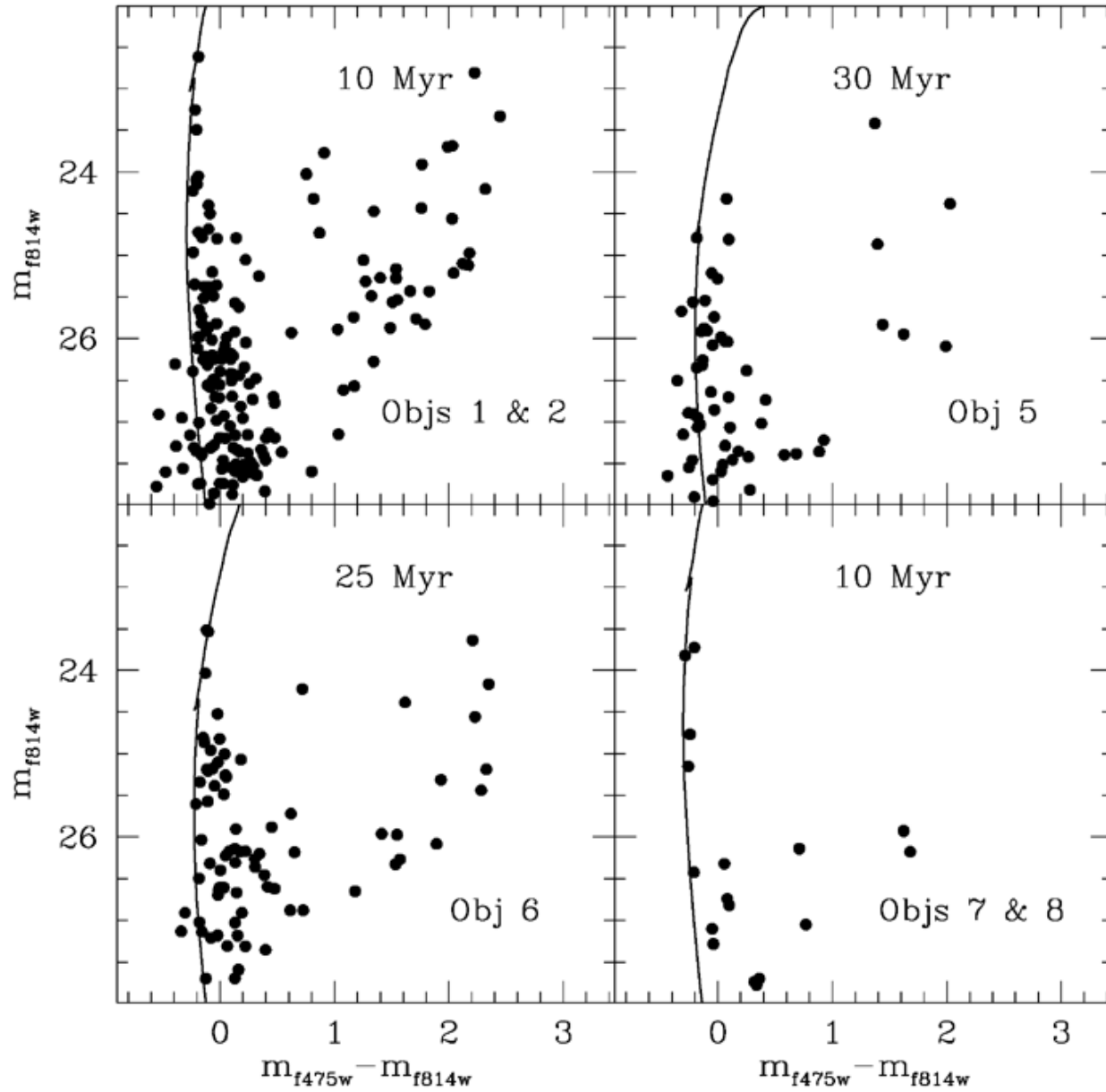
Figure 7. from Star Formation in the H I Bridge Between M81 and M82 DE MELLO ET AL. 2008 AJ 135 548 doi:10.1088/0004-6256/135/2/548 https://dx.doi.org/10.1088/0004-6256/135/2/548 © 2008. The American Astronomical Society. All rights reserved.
