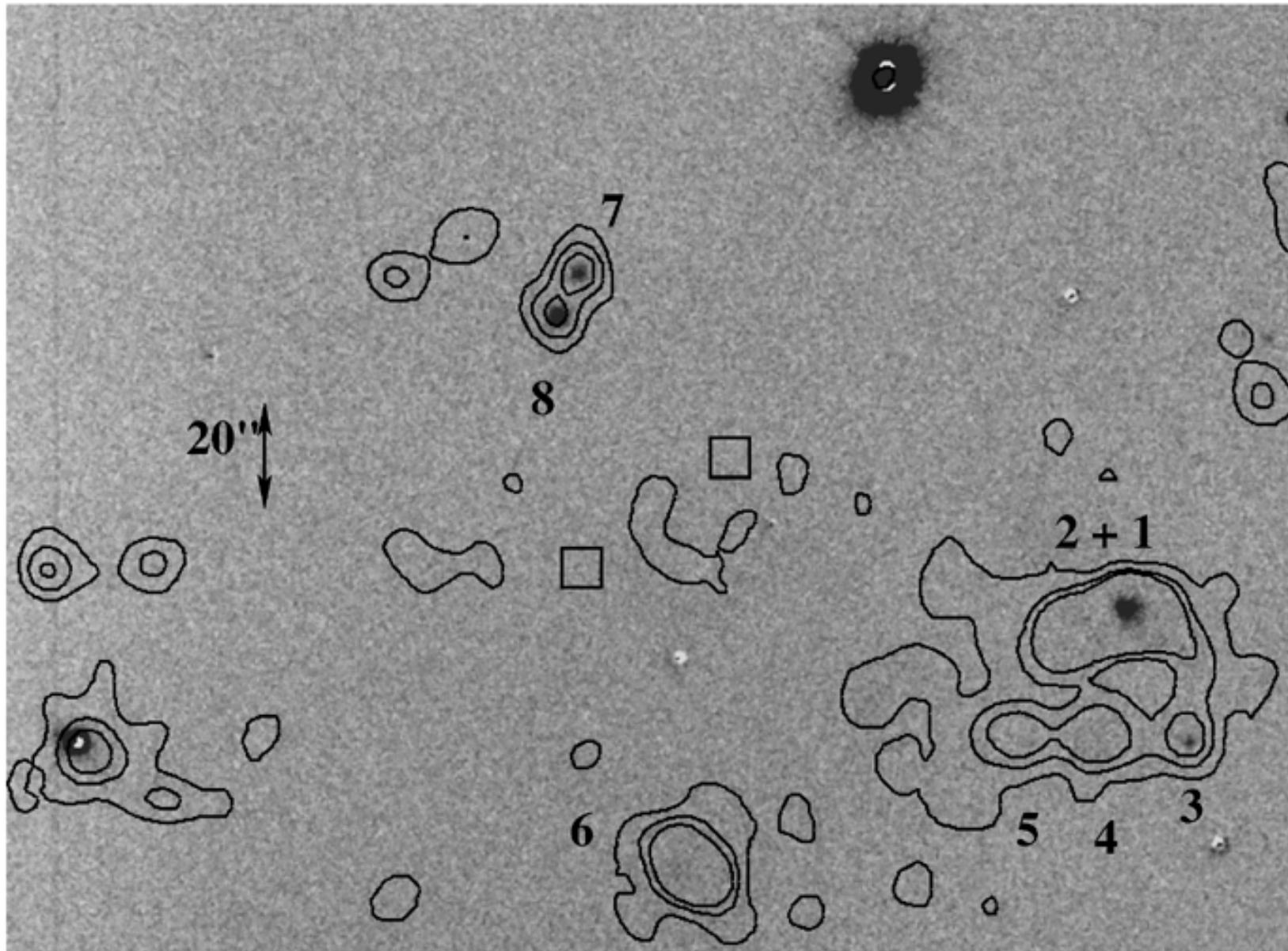
Figure 5. from Star Formation in the H I Bridge Between M81 and M82 DE MELLO ET AL. 2008 AJ 135 548 doi:10.1088/0004-6256/135/2/548 https://dx.doi.org/10.1088/0004-6256/135/2/548 © 2008. The American Astronomical Society. All rights reserved.
