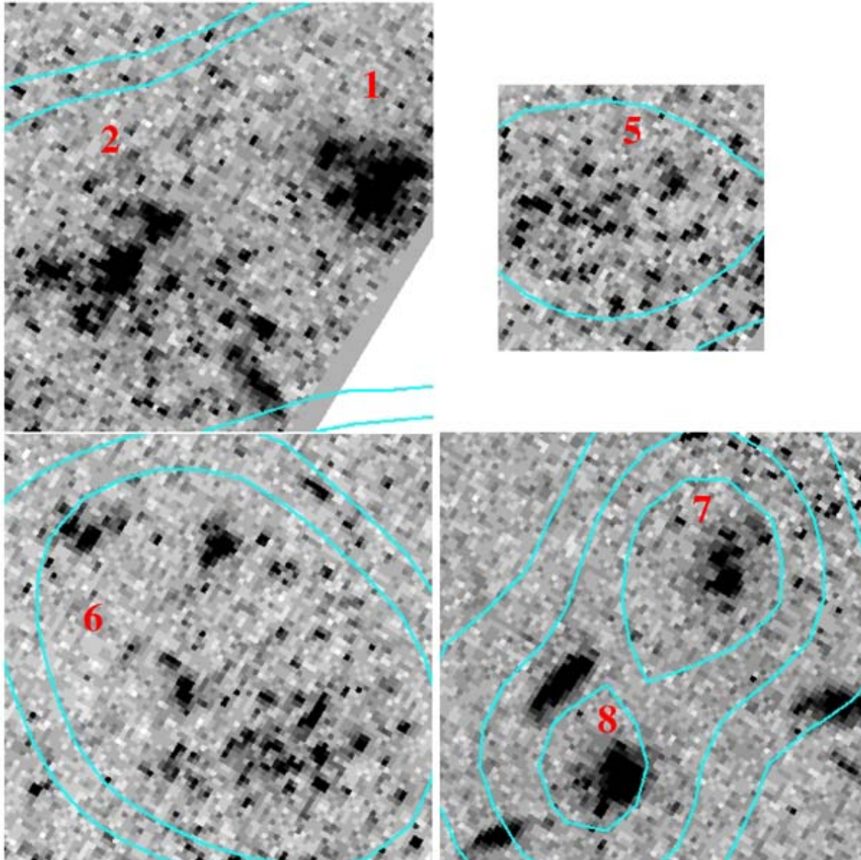
Figure 4. from Star Formation in the H I Bridge Between M81 and M82 DE MELLO ET AL. 2008 AJ 135 548 doi:10.1088/0004-6256/135/2/548 https://dx.doi.org/10.1088/0004-6256/135/2/548 © 2008. The American Astronomical Society. All rights reserved.
