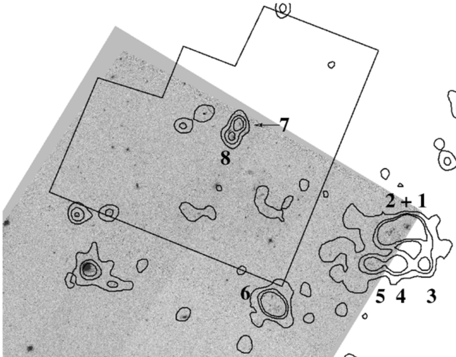
Figure 3. from Star Formation in the H I Bridge Between M81 and M82 DE MELLO ET AL. 2008 AJ 135 548 doi:10.1088/0004-6256/135/2/548 https://dx.doi.org/10.1088/0004-6256/135/2/548 © 2008. The American Astronomical Society. All rights reserved.
