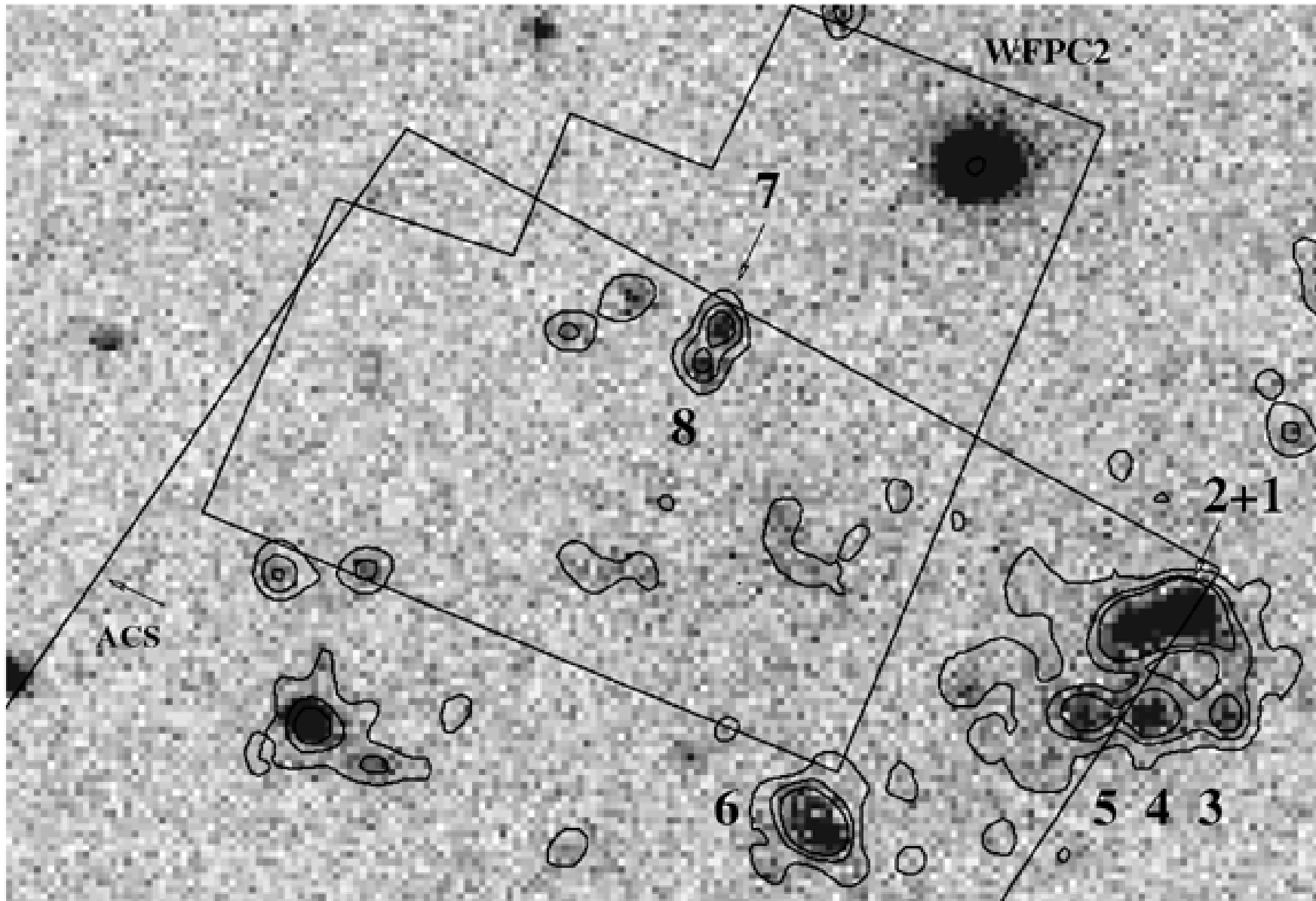
Figure 2. from Star Formation in the H I Bridge Between M81 and M82 DE MELLO ET AL. 2008 AJ 135 548 doi:10.1088/0004-6256/135/2/548 https://dx.doi.org/10.1088/0004-6256/135/2/548 © 2008. The American Astronomical Society. All rights reserved.
