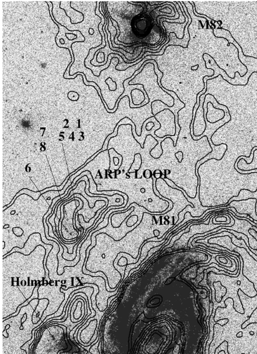
Figure 1. from Star Formation in the H I Bridge Between M81 and M82 DE MELLO ET AL. 2008 AJ 135 548 doi:10.1088/0004-6256/135/2/548 https://dx.doi.org/10.1088/0004-6256/135/2/548 © 2008. The American Astronomical Society. All rights reserved.
