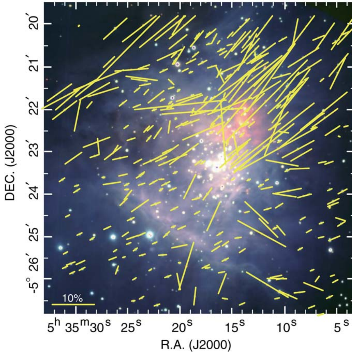
Figure 2. from Near-Infrared Imaging Polarimetry of M42: Aperture Polarimetry of Point-Like Sources KUSAKABE ET AL. 2008 AJ 136 621 doi:10.1088/0004-6256/136/2/621 https://dx.doi.org/10.1088/0004-6256/136/2/621 © 2008. The American Astronomical Society. All rights reserved.
