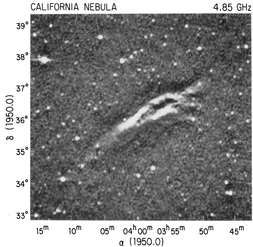
FIG. 10. A 4.85 GHz map centered on the California Nebula (NGC 1499).
