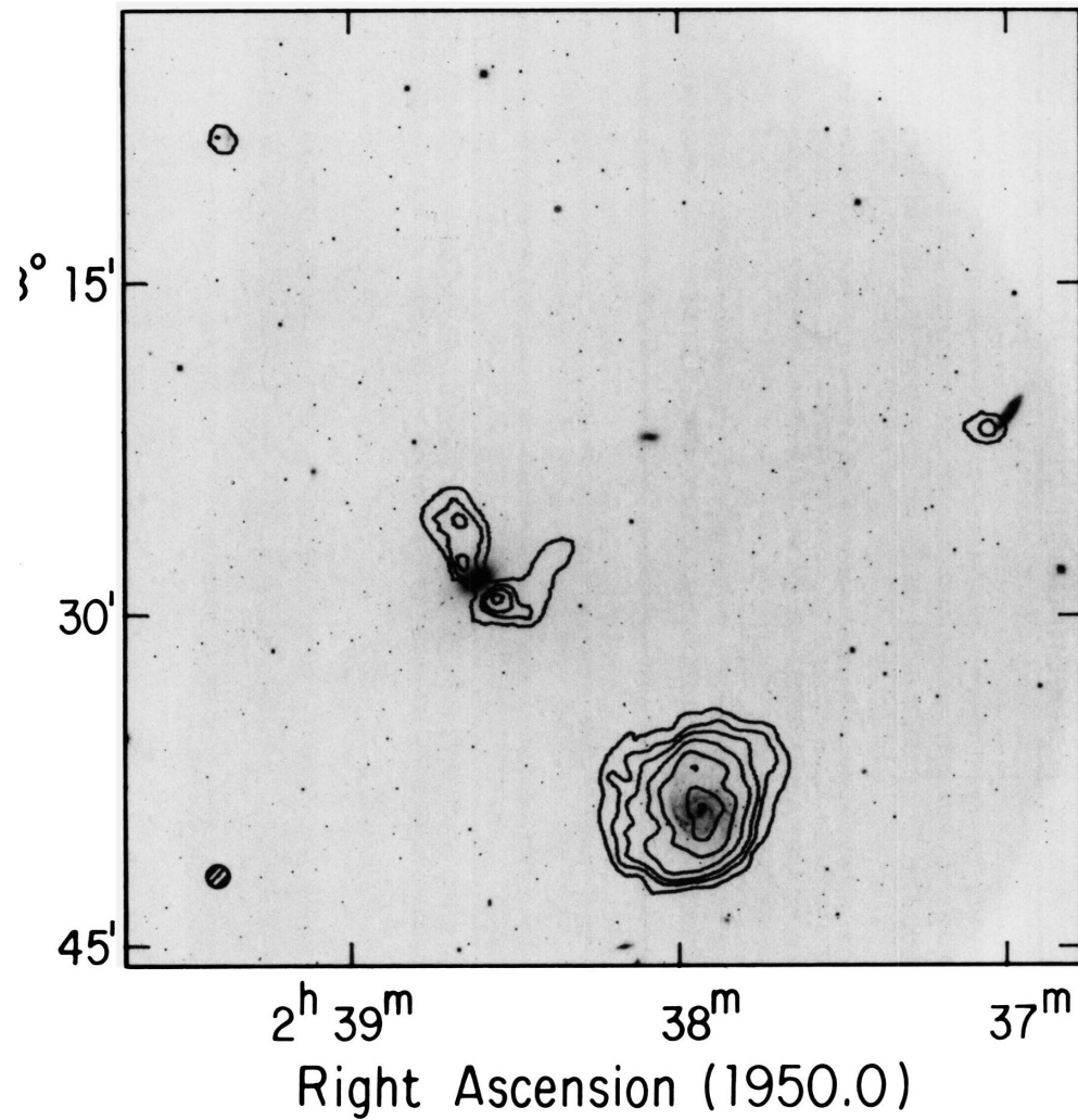
FIG. 13. Total H I map for the NGC 1052 group overlaid on a 4 m plate of the group.
