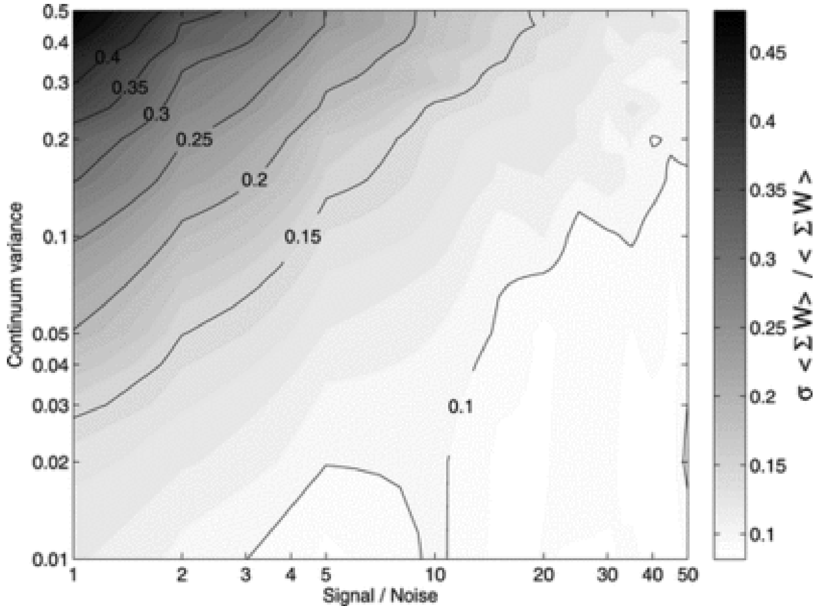
Fig. 8. from Kinematic and Chemical Constraints on the Formation of M31's Inner and Outer Halo Koch et al. 2008 ApJ 689 958 doi:10.1086/592373 https://dx.doi.org/10.1086/592373
