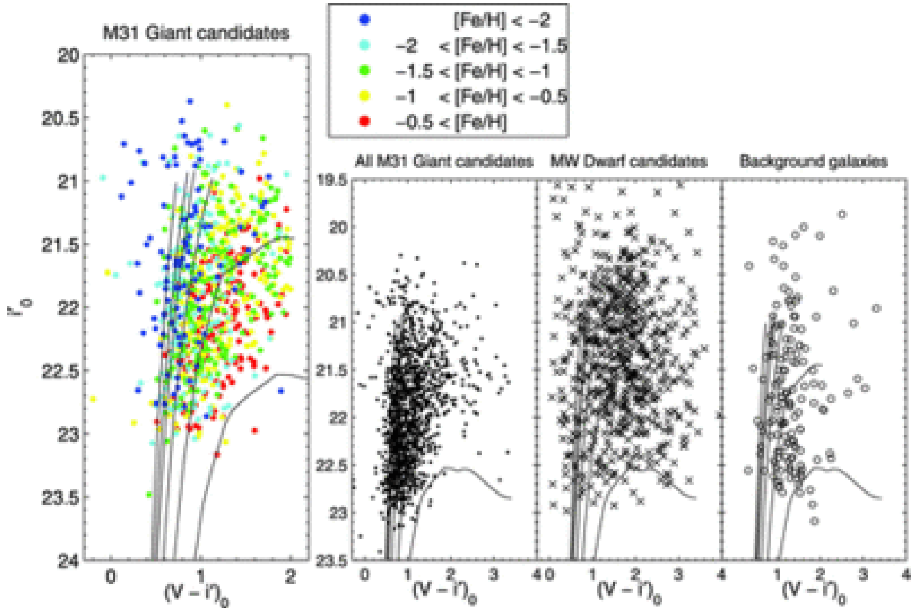
Fig. 3. from Kinematic and Chemical Constraints on the Formation of M31's Inner and Outer Halo Koch et al. 2008 ApJ 689 958 doi:10.1086/592373 https://dx.doi.org/10.1086/592373 © 2008. The American Astronomical Society. All rights reserved. Printed in U.S.A.
