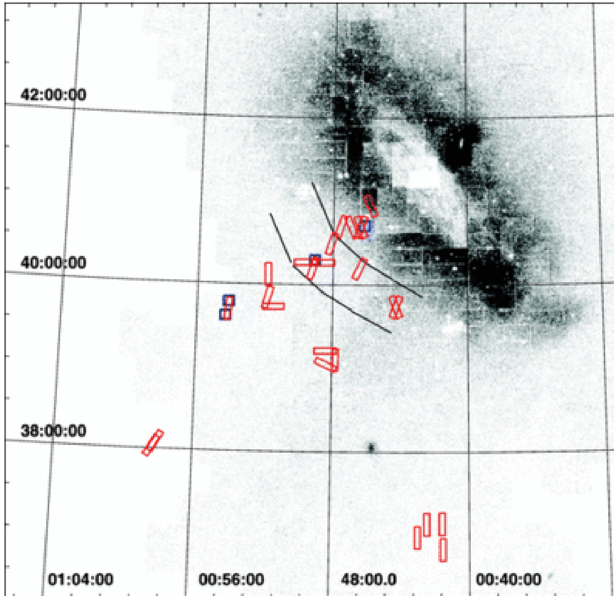
Fig. 1. from Kinematic and Chemical Constraints on the Formation of M31's Inner and Outer Halo Koch et al. 2008 ApJ 689 958 doi:10.1086/592373 https://dx.doi.org/10.1086/592373 © 2008. The American Astronomical Society. All rights reserved. Printed in U.S.A.
