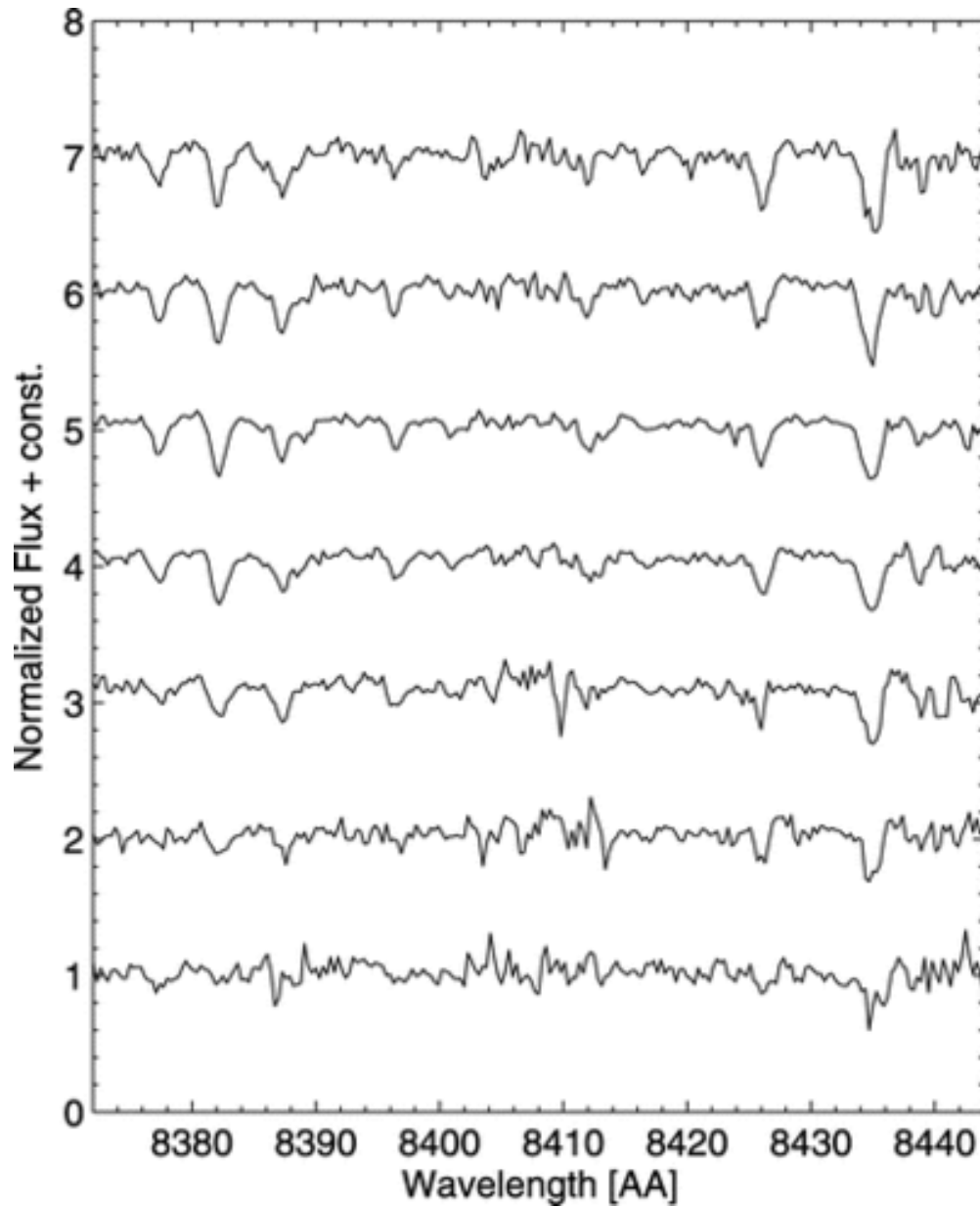
Fig. 17. from Kinematic and Chemical Constraints on the Formation of M31's Inner and Outer Halo Koch et al. 2008 ApJ 689 958 doi:10.1086/592373 https://dx.doi.org/10.1086/592373
