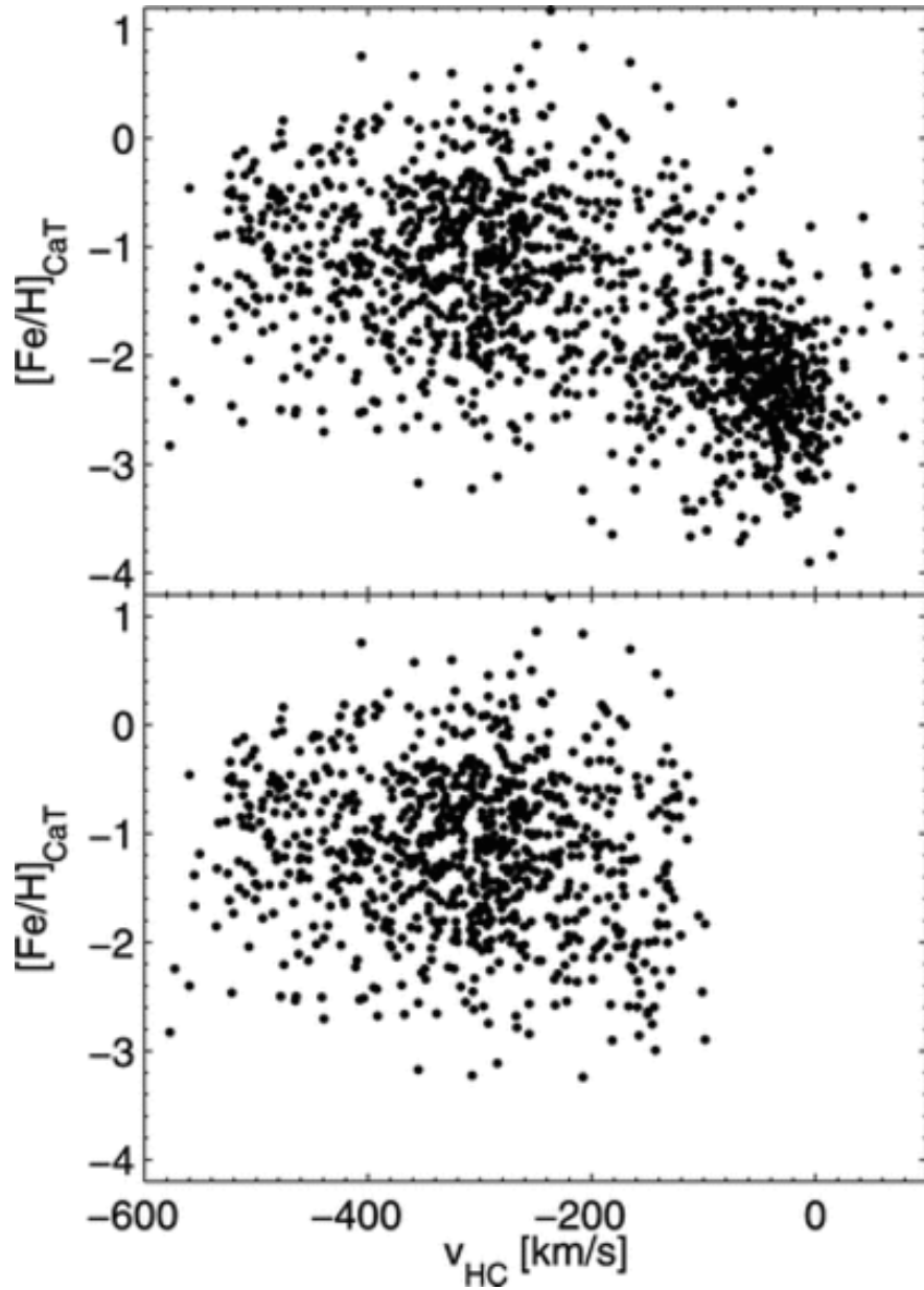
Fig. 14. from Kinematic and Chemical Constraints on the Formation of M31's Inner and Outer Halo Koch et al. 2008 ApJ 689 958 doi:10.1086/592373 https://dx.doi.org/10.1086/592373 © 2008. The American Astronomical Society. All rights reserved. Printed in U.S.A.
