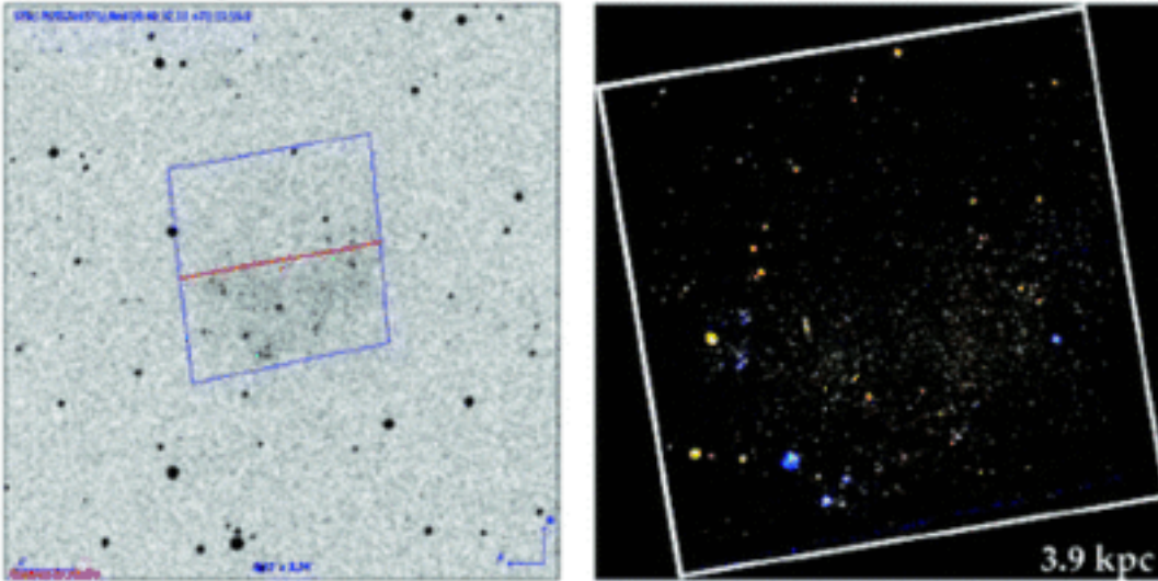
(a) DSS Image with ACS Footprint (b) ACS Field of Ho I
