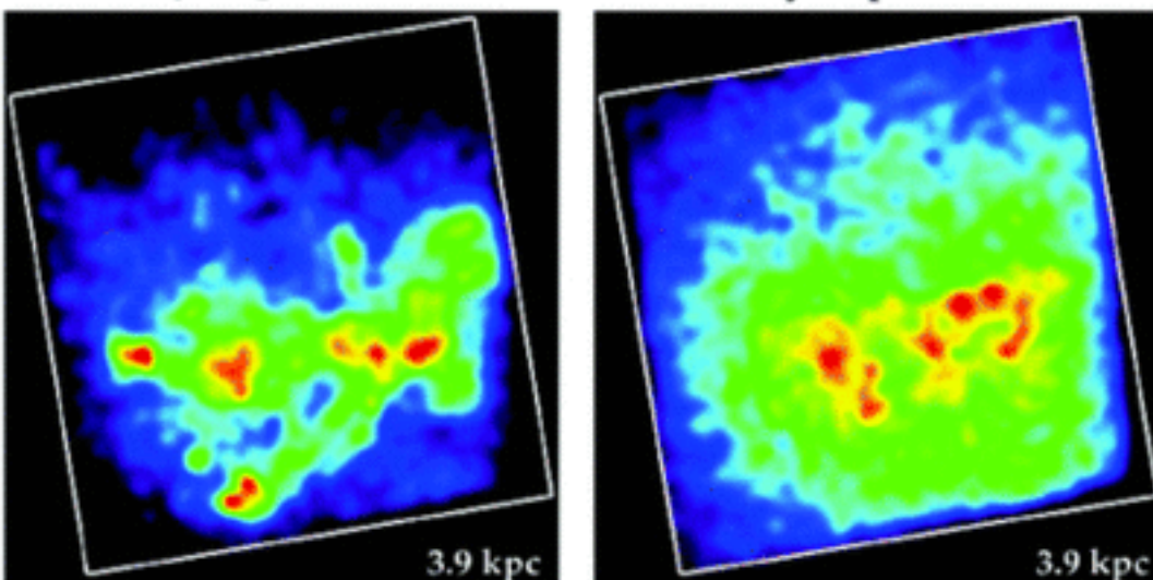
(c) Density Map of Blue Stars (d) Density Map of Red Stars
