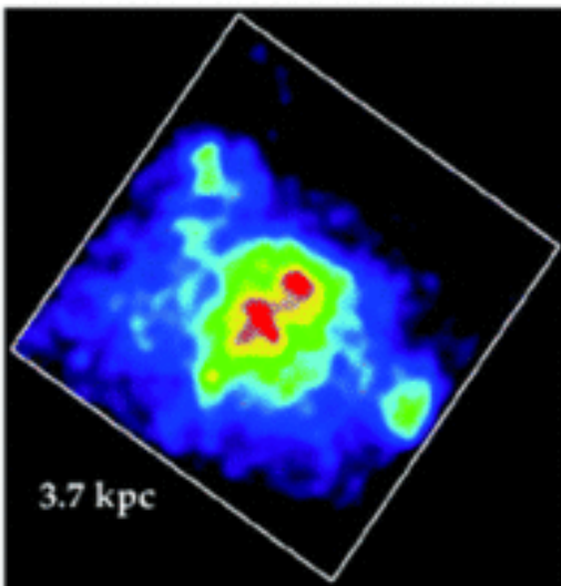
(c) Density Map of Blue Stars
