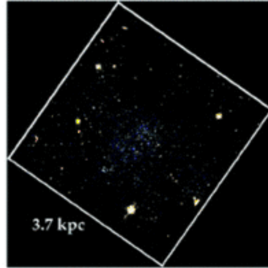
(a) DSS Image with ACS Footprint (b) ACS Field of Ho IX
