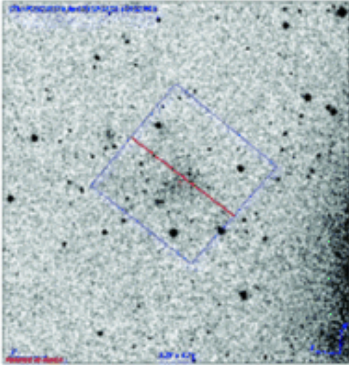
(a) DSS Image with ACS Footprint (b) ACS Field of Ho IX
