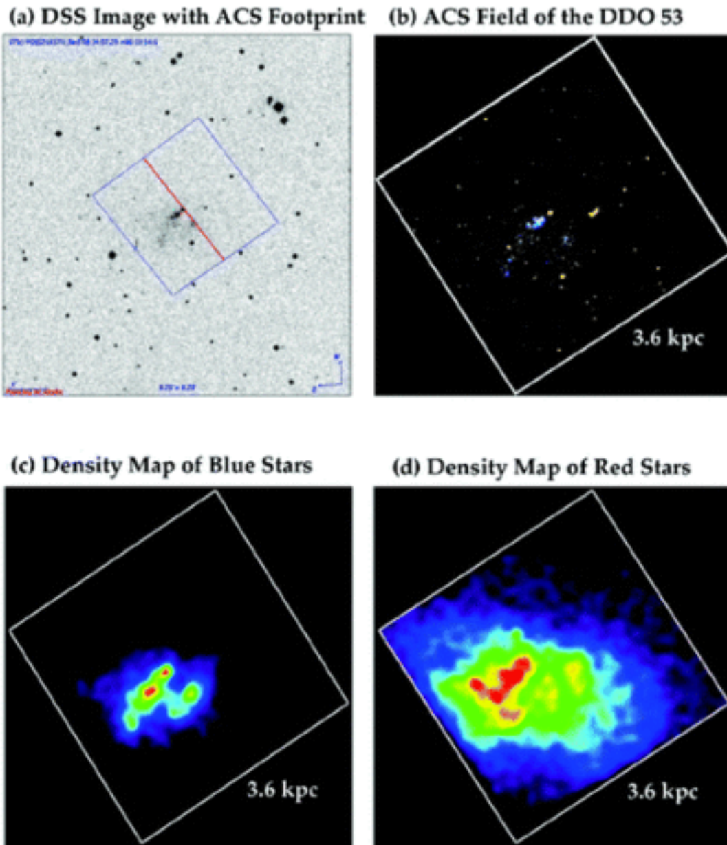
Fig. 7. from The Recent Star Formation Histories of M81 Group Dwarf Irregular Galaxies Weisz et al. 2008 ApJ 689 160 doi:10.1086/592323 https://dx.doi.org/10.1086/592323 Copyright is not claimed for this article. Printed in U.S.A.
