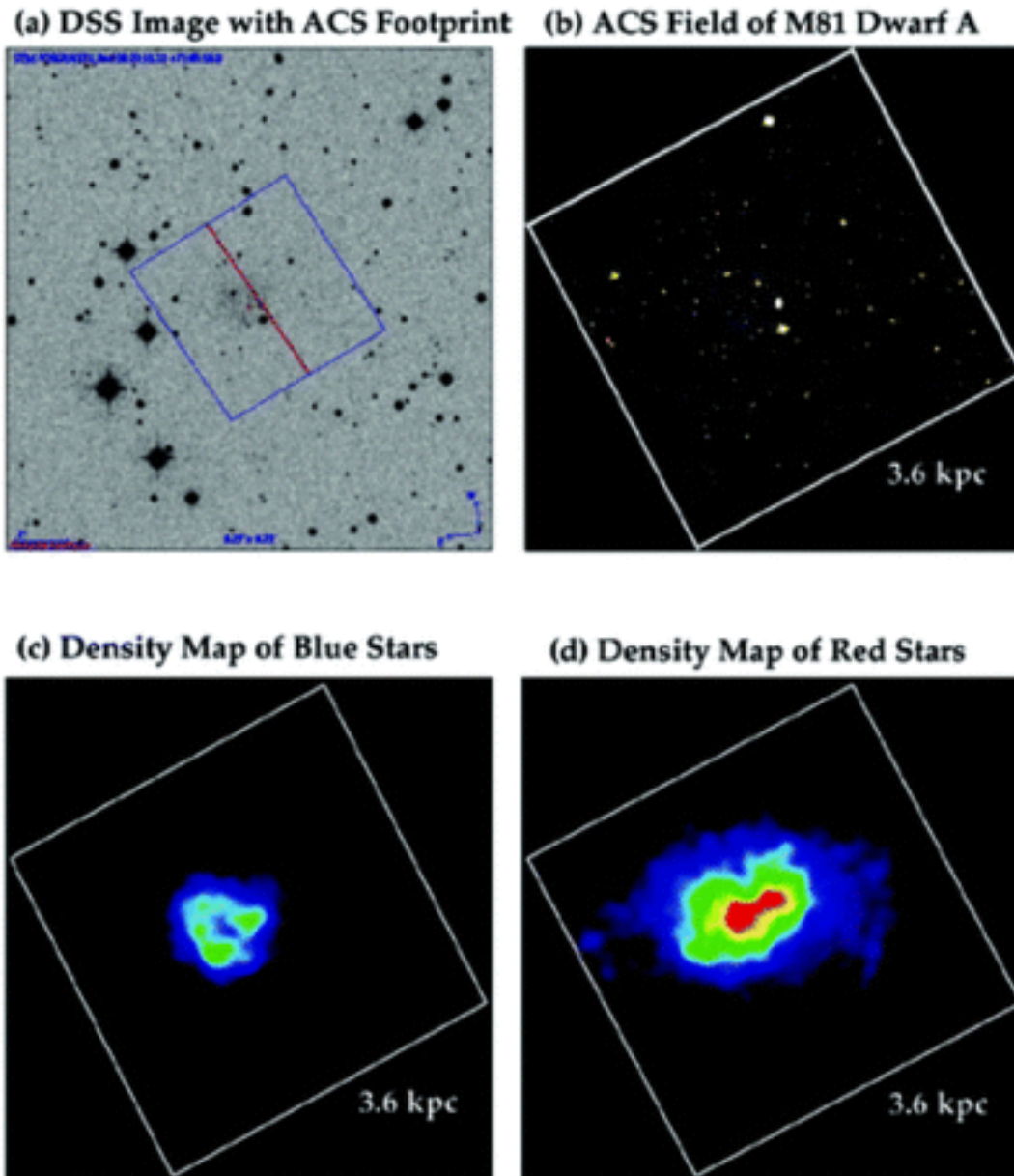
Fig. 6. from The Recent Star Formation Histories of M81 Group Dwarf Irregular Galaxies Weisz et al. 2008 ApJ 689 160 doi:10.1086/592323 https://dx.doi.org/10.1086/592323 Copyright is not claimed for this article. Printed in U.S.A.
