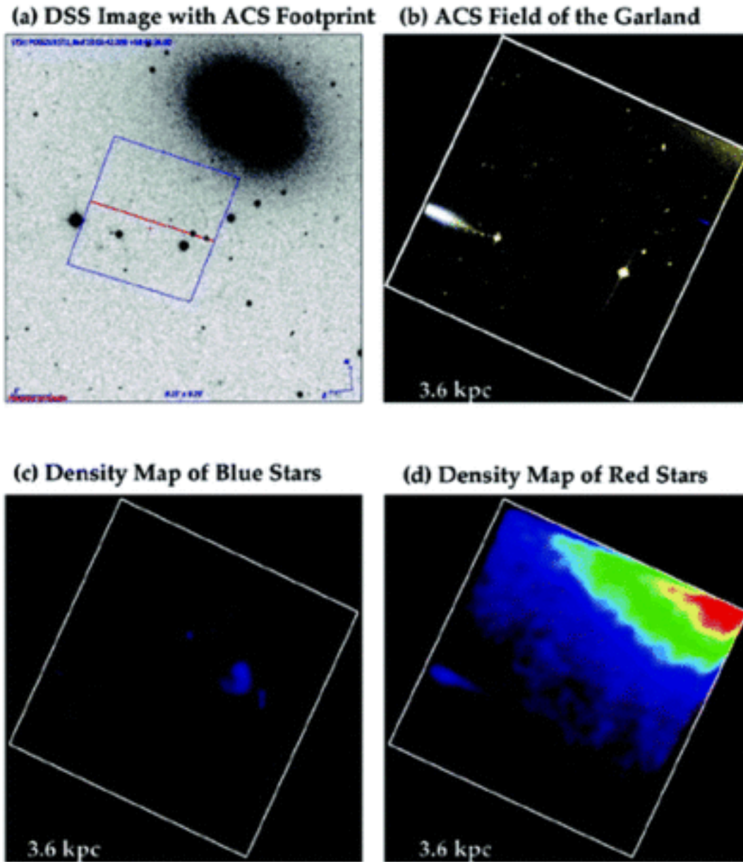
Fig. 5. from The Recent Star Formation Histories of M81 Group Dwarf Irregular Galaxies Weisz et al. 2008 ApJ 689 160 doi:10.1086/592323 https://dx.doi.org/10.1086/592323 Copyright is not claimed for this article. Printed in U.S.A.
