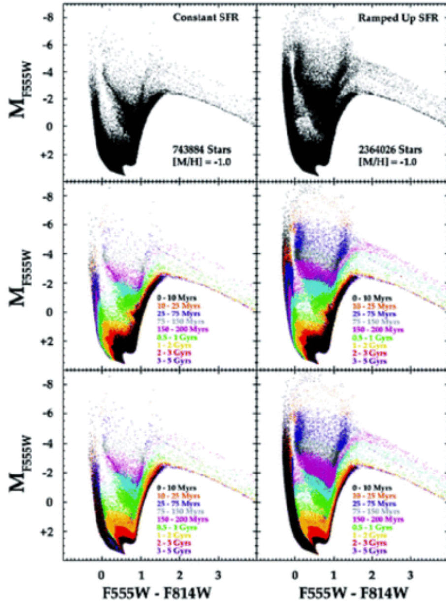
Fig. 4. from The Recent Star Formation Histories of M81 Group Dwarf Irregular Galaxies Weisz et al. 2008 ApJ 689 160 doi:10.1086/592323 https://dx.doi.org/10.1086/592323 Copyright is not claimed for this article. Printed in U.S.A.
