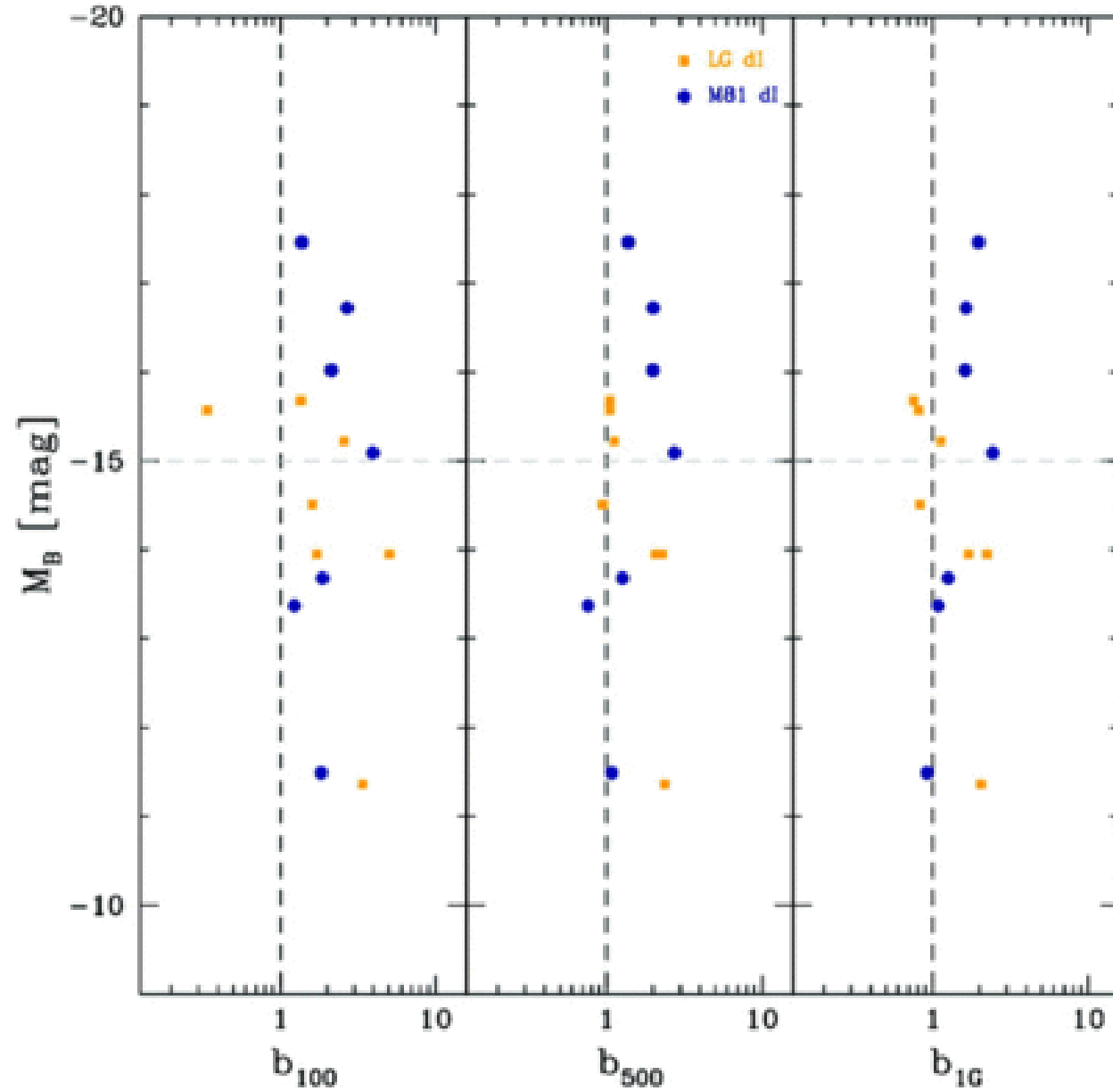
Fig. 23. from The Recent Star Formation Histories of M81 Group Dwarf Irregular Galaxies Weisz et al. 2008 ApJ 689 160 doi:10.1086/592323 https://dx.doi.org/10.1086/592323 Copyright is not claimed for this article. Printed in U.S.A.
