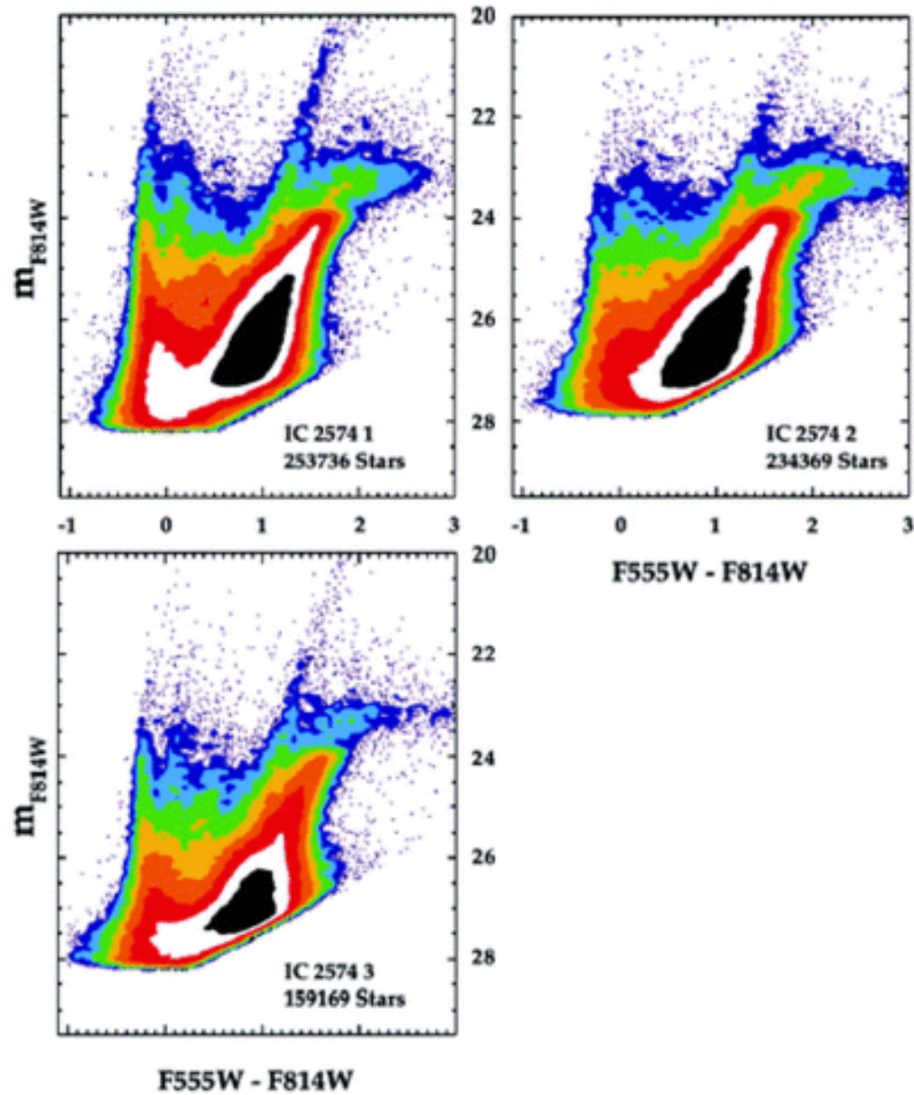
Fig. 17. from The Recent Star Formation Histories of M81 Group Dwarf Irregular Galaxies Weisz et al. 2008 ApJ 689 160 doi:10.1086/592323 https://dx.doi.org/10.1086/592323 Copyright is not claimed for this article. Printed in U.S.A.
