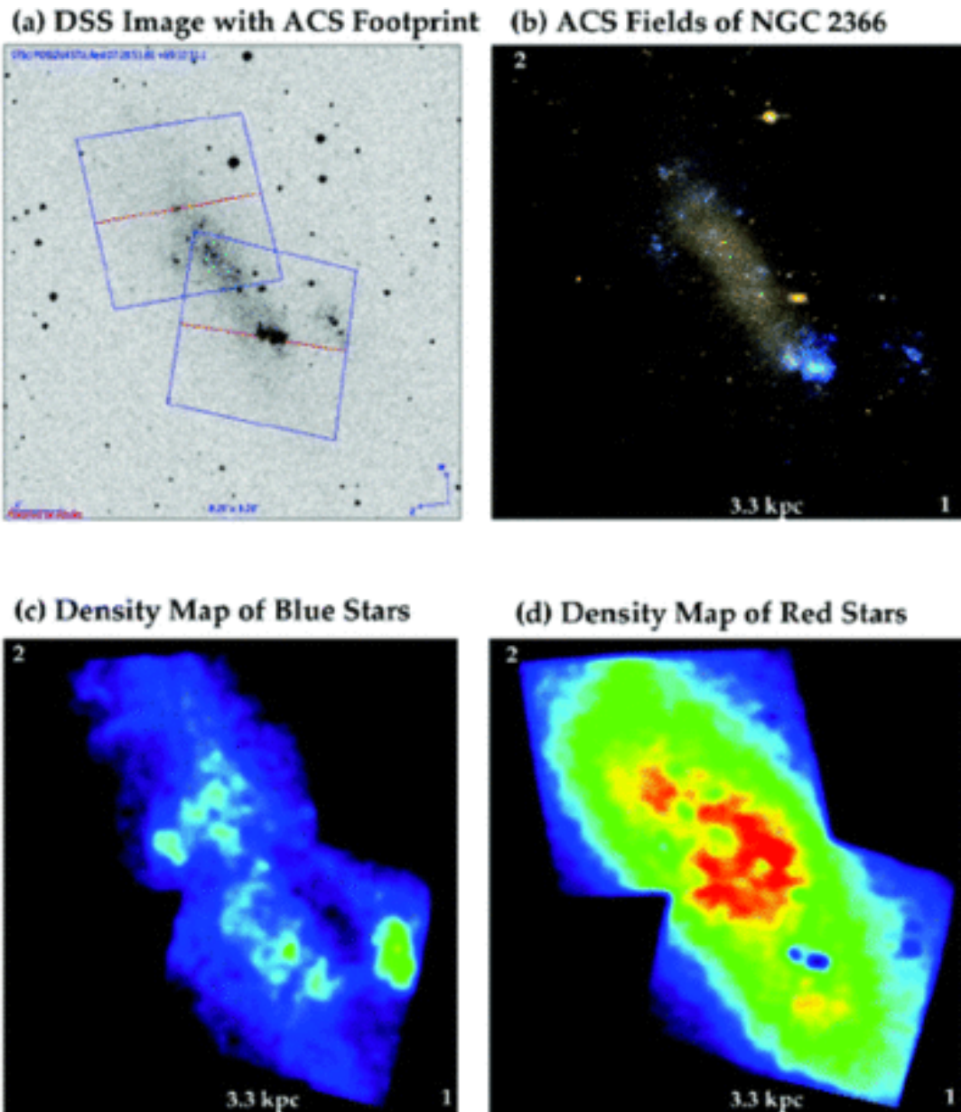
Fig. 11. from The Recent Star Formation Histories of M81 Group Dwarf Irregular Galaxies Weisz et al. 2008 ApJ 689 160 doi:10.1086/592323 https://dx.doi.org/10.1086/592323 Copyright is not claimed for this article. Printed in U.S.A.
