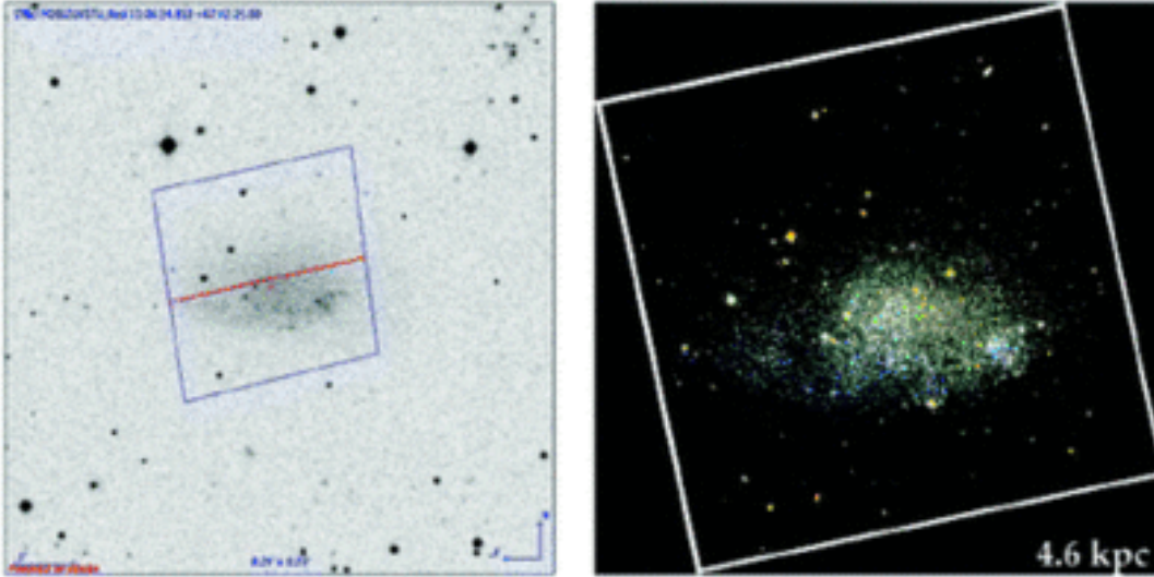
(a) DSS Image with ACS Footprint (b) ACS Field of DDO 165
