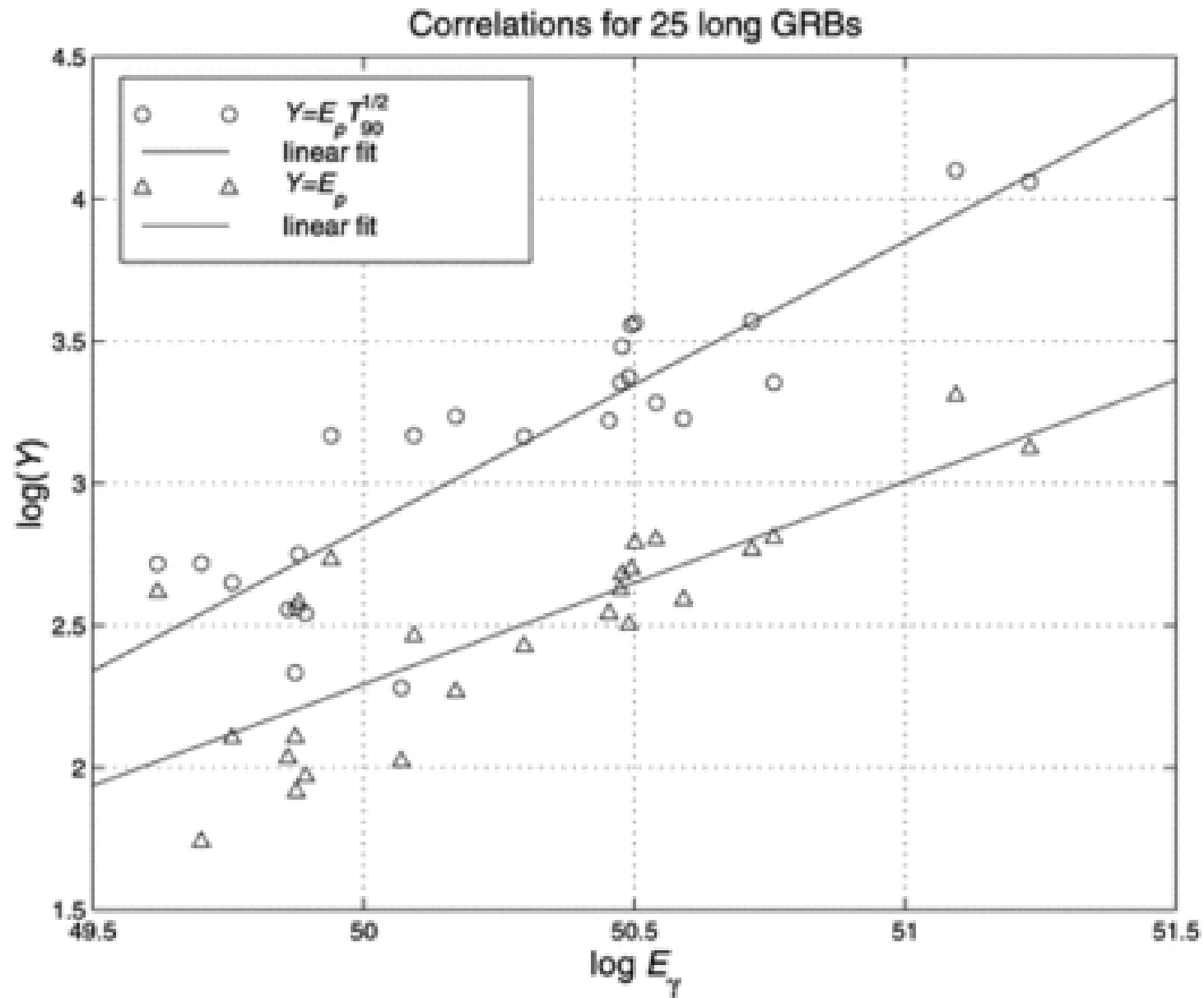
Fig. 1. from Nonthermal HighEnergy Emissions from Black Holes by a Relativistic Capillary Effect van Putten 2008 ApJL 685 L63 doi:10.1086/592293 https://dx.doi.org/10.1086/592293 © 2008. The American Astronomical Society. All rights reserved. Printed in U.S.A.
