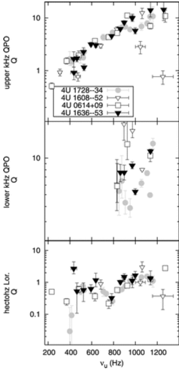
Fig. 12. from XRay Time Variability Across the Atoll Source States of 4U 163653 Altamirano et al. 2008 ApJ 685 436 doi:10.1086/590897 https://dx.doi.org/10.1086/590897 © 2008. The American Astronomical Society. All rights reserved. Printed in U.S.A.
