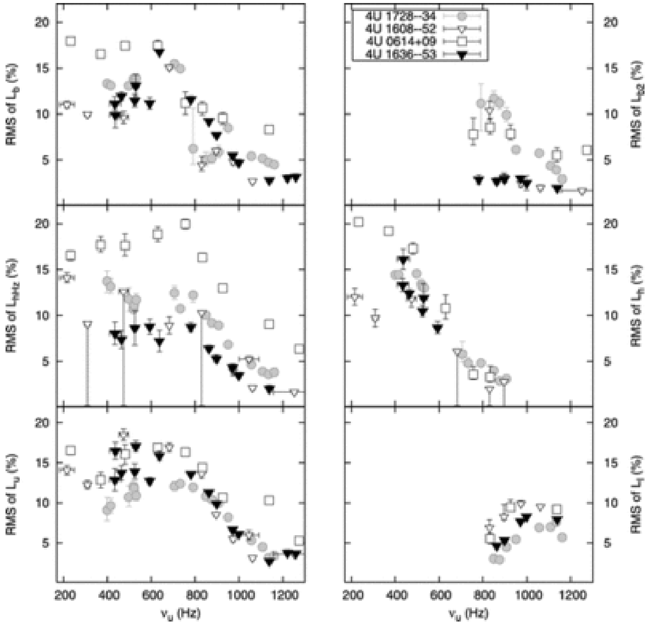
Fig. 11. from XRay Time Variability Across the Atoll Source States of 4U 163653 Altamirano et al. 2008 ApJ 685 436 doi:10.1086/590897 https://dx.doi.org/10.1086/590897 © 2008. The American Astronomical Society. All rights reserved. Printed in U.S.A.
