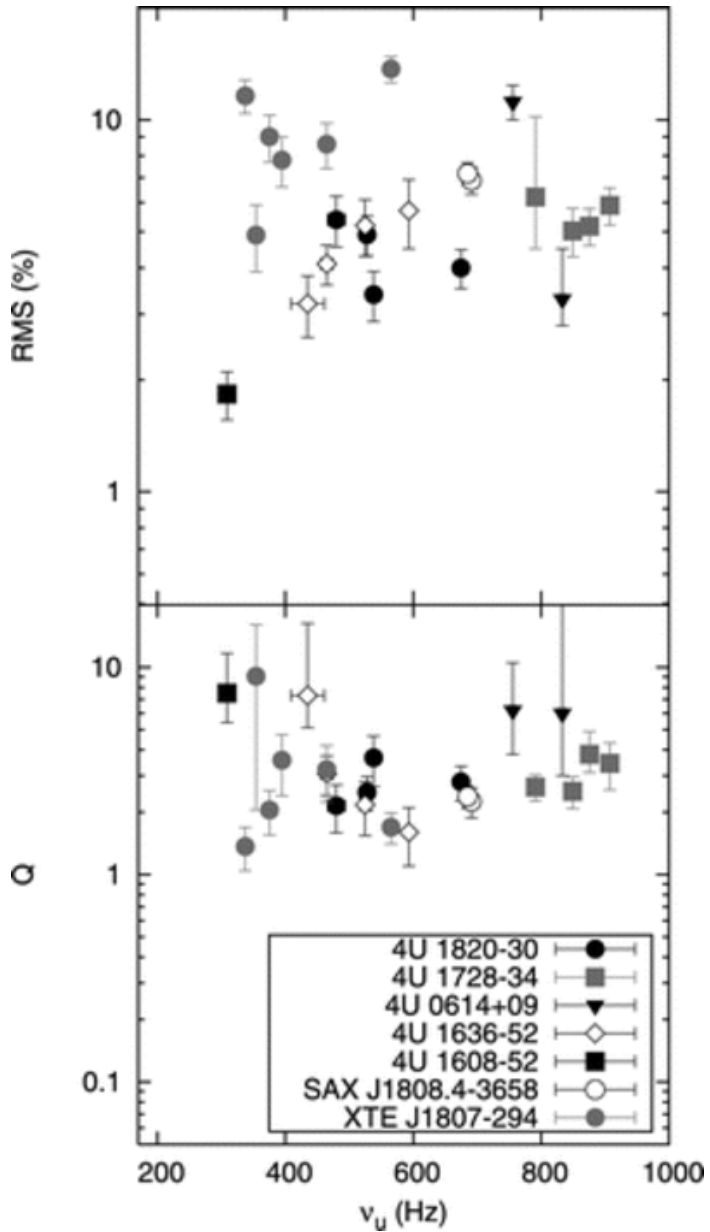
Fig. 10. from XRay Time Variability Across the Atoll Source States of 4U 163653 Altamirano et al. 2008 ApJ 685 436 doi:10.1086/590897 https://dx.doi.org/10.1086/590897 © 2008. The American Astronomical Society. All rights reserved. Printed in U.S.A.
