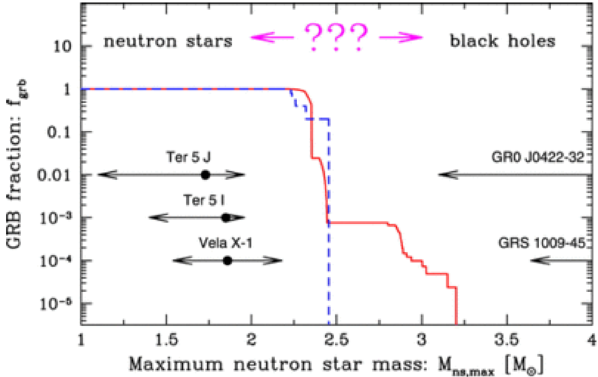
Fig. 4. from The Lowest Mass Stellar Black Holes: Catastrophic Death of Neutron Stars in GammaRay Bursts Belczynski et al. 2008 ApJL 680 L129 doi:10.1086/589970 https://dx.doi.org/10.1086/589970 © 2008. The American Astronomical Society. All rights reserved. Printed in U.S.A.
